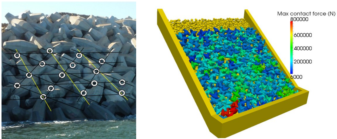
Figure 2. Left: breakwater trunk section of CORE-LOC™ concrete units, built to a designated packing density with rules adopted to achieve good interlocking. Right: model of 242 Core-Loc units of 8\text{m}^3 volume with colour key indicating maximum contact forces on each unit. These are generally higher in the toe rows and in the example shown, force chains can be observed.
