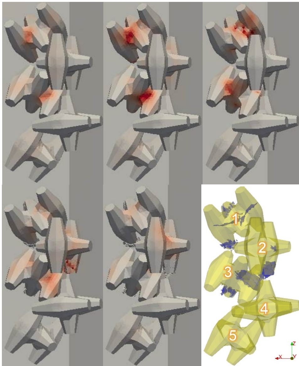
Figure 14 Numerical simulation results of interaction between CORE-LOC™ units under gravity on a sloping base, sequence at t=0.061, 0.063, 0.067, 0.084, and 0.1 seconds, showing maximum principal stress \sigma_1 where tensile stress is positive, (engineering stress convention). The final image shows 3D fractures.
