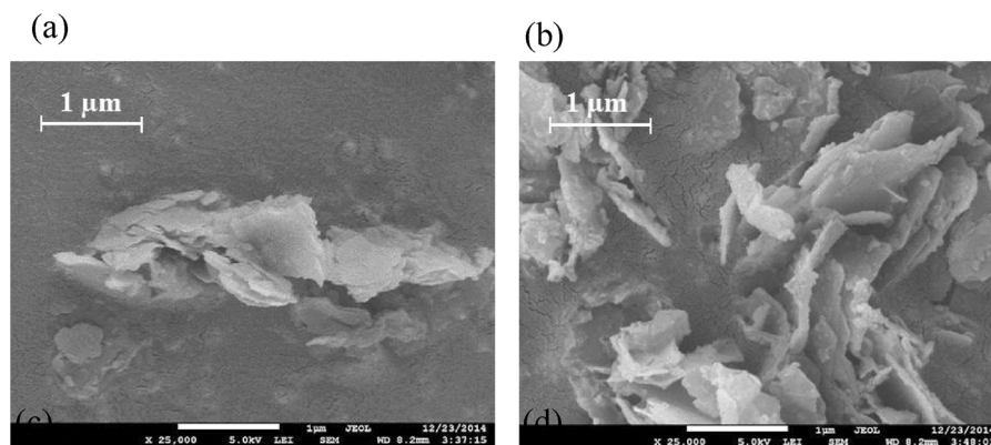
Fig. 5. SEM micrographs of un-doped (a) and MBT-doped (b) Zn-Al LDHs at 25000x.
