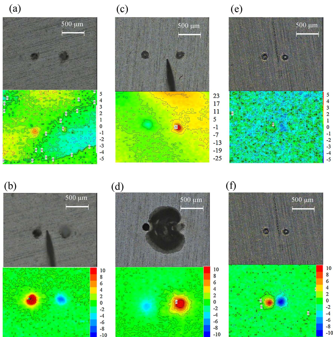
Fig. 10. Optical micrographs and SVET maps of Ep-NaY-Ce (a) and (b), Ep-LDH-MBT (c) and (d) and Ep-NaY-Ce_LDH-MBT (e) and (f) after 1 (a, c, e) and 7 (b, d, f) days exposure to 0.05 M NaCl. (For interpretation of the references to colour, the reader is referred to the web version of this article.)
