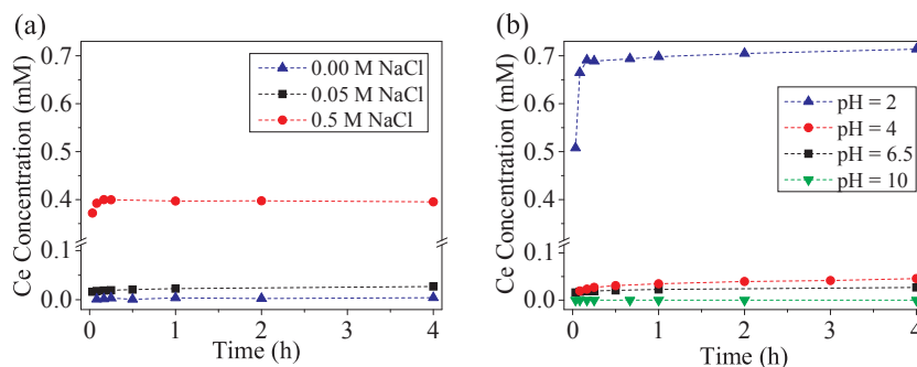
Fig. 6. \text{Ce}^{3+} release profiles at neutral pH in different NaCl concentrations (a) and in 0.05 M NaCl at different pH values (b).
