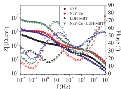
Fig. 8. EIS spectra of waterborne epoxy coatings after 7 days exposure to 0.05 M NaCl.
