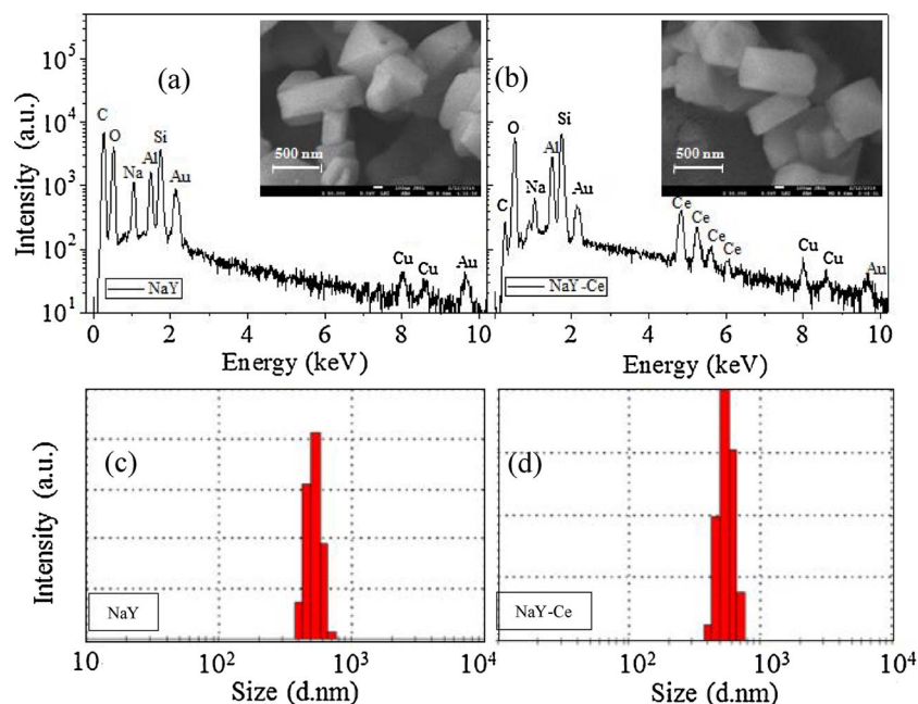
Fig. 4. EDS spectra and SEM micrographs (picture inset) of NaY (a) and NaY-Ce and size distribution of NaY (c) and NaY-Ce particles (d).
