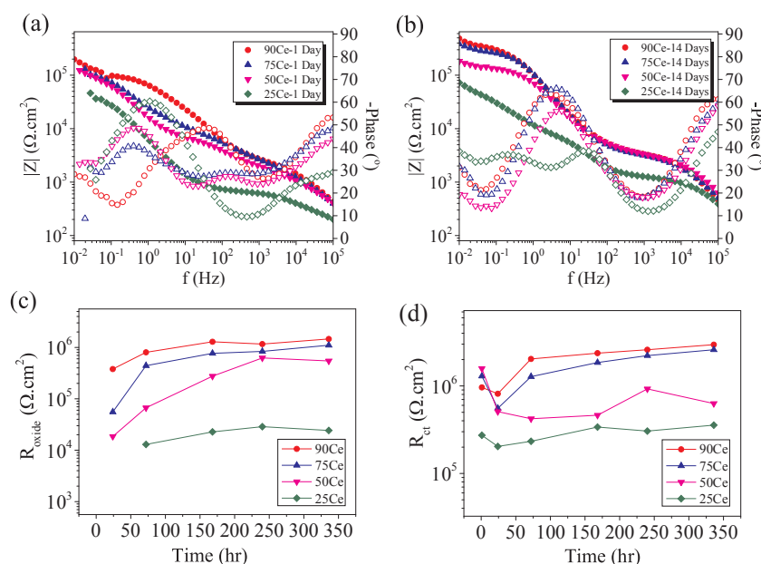
Fig. 12. The EIS spectra of the epoxy coatings containing different ratios of NaY-Ce:LDH-MBT after 1 day (a) and 14 days (b) and the evolution of R_{oxide} (c) and R_{ct} (d) of the coating systems in 0.05 M NaCl. (90Ce, 75Ce, 50Ce and 25Ce represent NaY-Ce:LDH-MBT ratios of 90:10, 75:25, 50:50 and 25:75, respectively).
