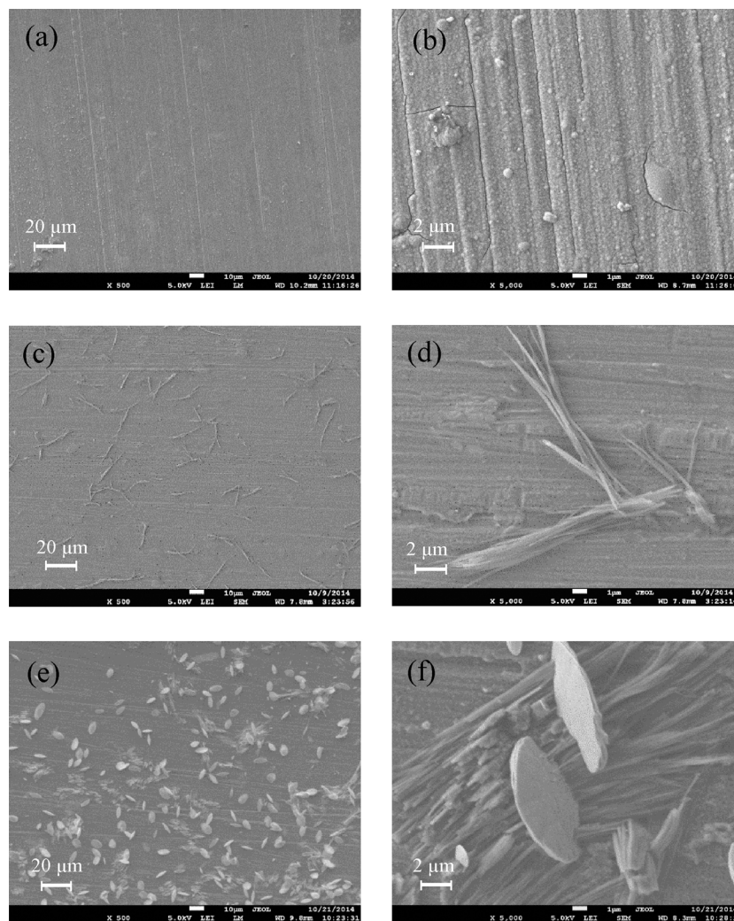
Fig. 2. SEM micrographs of AA2024-T3 exposed for 14 days to 1 mM \text{Ce}(\text{NO}_3)_3 at 500x (a) and 5000x (b), to 1 mM MBT at 500x (c) and 5000x (d) and to 0.5 mM \text{Ce}(\text{NO}_3)_3 + 0.5 mM MBT at 500x (e) and 5000x (f).
