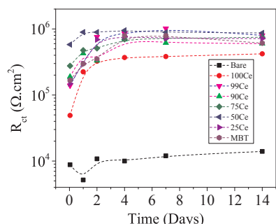
Fig. 3. Evolution of the R_{ct} of AA2024-T3 panels in 0.05 M NaCl solution containing different Ce^{3+} :MBT molar ratios.
