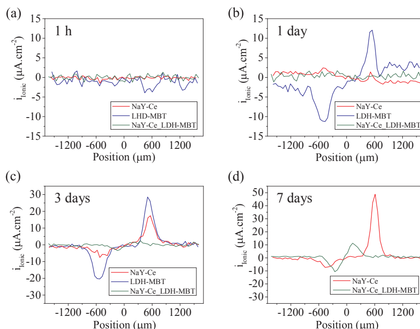
Fig. 11. Ionic current density profiles of the extrinsic healing corrosion protective epoxy coatings after 1 h (a), 1 day (b), 3 days (c) and 7 days (d) exposure to 0.05 M NaCl, respectively.
