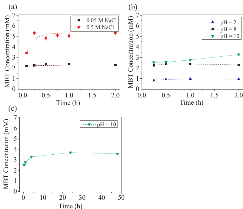
Fig. 7. MBT release profiles at neutral pH in different NaCl concentrations (a) and in 0.05 M NaCl at different pH values (b).
