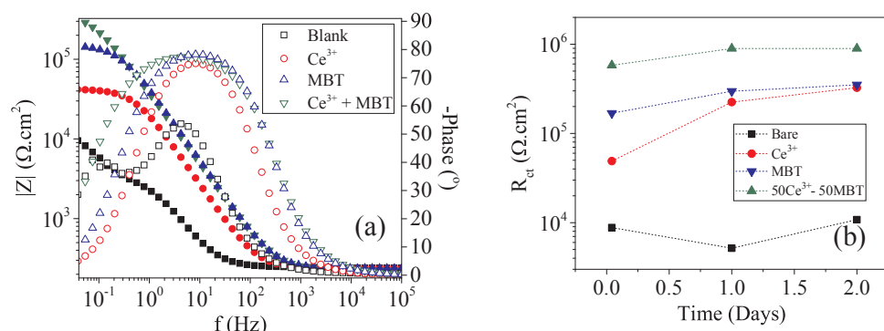
Fig. 1. The EIS spectra after 60 min immersion (a) and evolution of the R_{ct} for AA2024-T3 panels exposed to inhibitor free (■), 1 mM \text{Ce}^{3+} (●), 1 mM MBT (▼) and 0.5 mM \text{Ce}^{3+} + 0.5 mM MBT (▲) containing 0.05 M NaCl (b).
