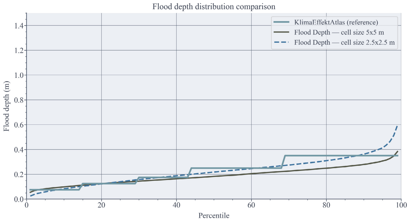
Figure 70. Percentile value comparison between simulation result with cell 5 × 5 m, cell 2.5 × 2.5 m, and Climate Impact Atlas Map
