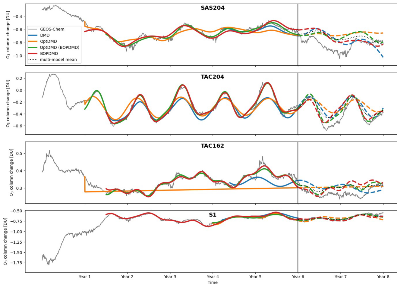
Figure A3. Selection of DMD models identified by the hyperparameter sweep, selected for the best 2-year forecast performance for the SAS204, TAC204, TAC162, and S1 scenarios. The rank and the length of fitting data is allowed to vary between the configurations, therefore the selected best results have different ranks and ranges of fitting data. In some cases however, such as for OptDMD with the TAC162 scenario, suitable configurations could still not be found.
