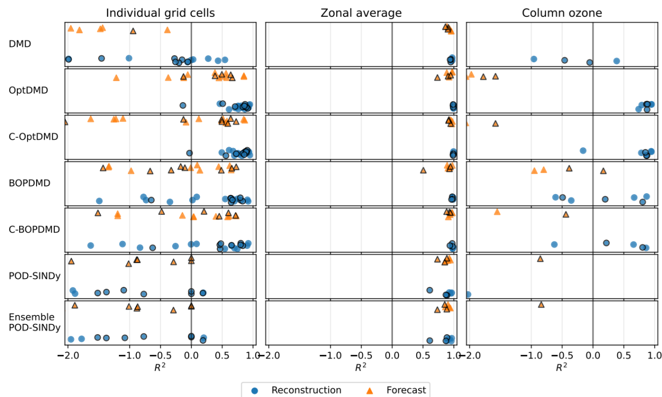
Figure C9. Comparison of the coefficient of determination for the single-cell (left panels), zonal-average (middle panels), and column ozone response (right panels). Reconstructions (blue) and forecasts (orange) are shown separately for the individual methods across all datasets.
