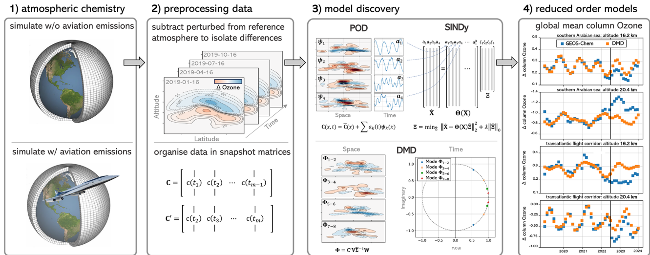
Figure 1. Methodology overview. In step 1 the effects of emissions are isolated by combining two GEOS-Chem atmosphere simulations, of which one is affected by the additional emissions. The resulting spatiotemporal datasets describe the daily average changes in ozone mass distribution for a period of 10 years. In step 2 the data is preprocessed and organised as a snapshot of matrices prior to applying data-driven methods (step 3). In step 4 the data-driven methods are used to forecast future behaviour of the ozone response, based on which the data-driven methods are assessed.
