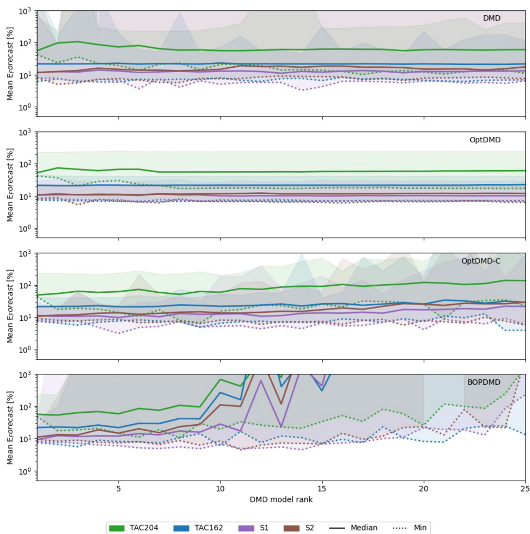
Figure A1. Results of hyperparameter sweep of DMD methods over the DMD rank, for the TAC204, TAC162, S1, and S2 emission scenario datasets. The solid lines indicate the median O 3 column change forecast error in percent. The shaded areas mark the full range of the error distribution, and the dotted lines mark the lowest forecast error achieved by any of the tried configurations.
