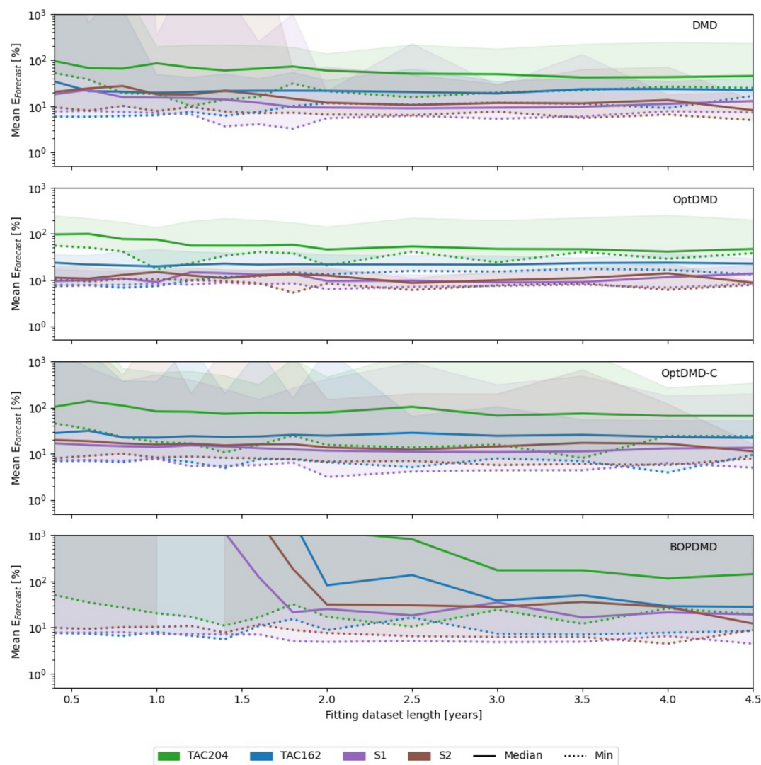
Figure A2. Results of hyperparameter sweep of DMD methods over the fitting dataset length, for the TAC204, TAC162, S1, and S2 emission scenario datasets. The solid lines indicate the median O_3 column change forecast error in percent. The shaded areas mark the full range of results, and the dotted lines mark the lowest forecast errors achieved by any of the tried configurations.
