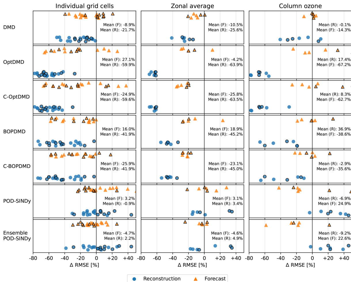
Figure 5. Change in the reconstruction (blue) and forecast (orange) RMSE with respect to reconstruction and forecasts using the temporal mean over all datasets for the methods used in this work. The left column shows the reconstruction of individual grid cells at altitudes of 1, 16, and 26 km (Table B1), the middle column the zonal average (Table 1), and the rightmost column the estimation of column ozone (Table 2). Markers with a black border denote the S1, S2, or S3 datasets.
