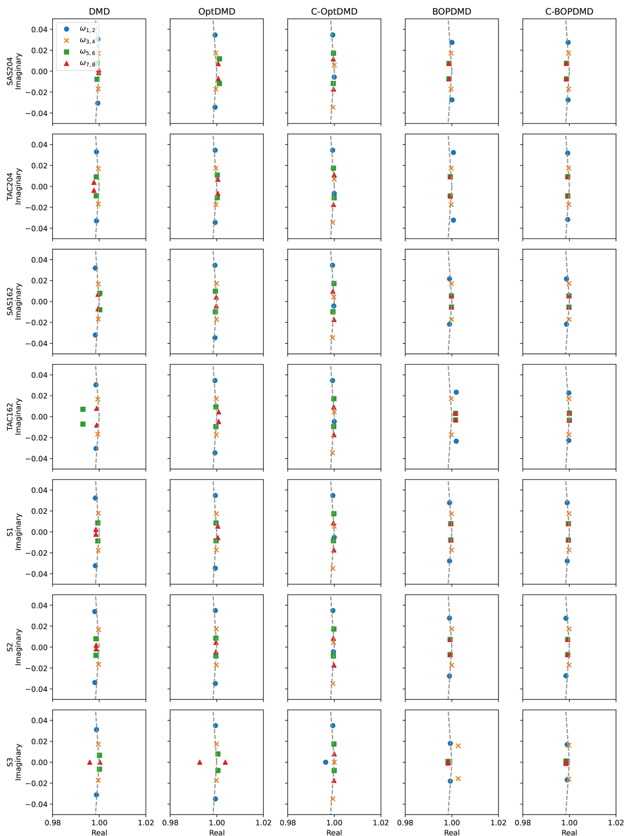
Figure C2. Eigenvalues of the conjugate pairs for the first four modes for each of the DMD variants applied to the different datasets. Markers show the conjugate pairs of the modes, and the dashed line shows the unit circle.
