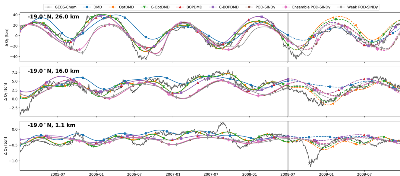
Figure C6. Same as Fig. C3, but for the S1 dataset.
