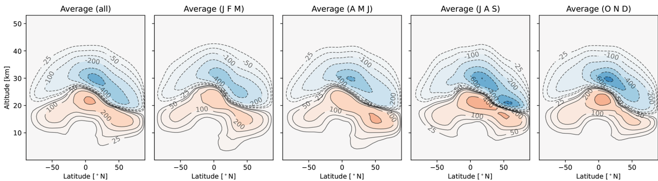
Figure 2. Average ozone response of the TAC204 dataset over different timespans in tons of ozone. The leftmost plot shows the average response over all 5 years of data, and the other four show averages taken over 3-monthly snapshots from the entire dataset. For example, the rightmost figure (Average (OND)) shows the average ozone response for the months of October, November, and December across the 5 years of data.
