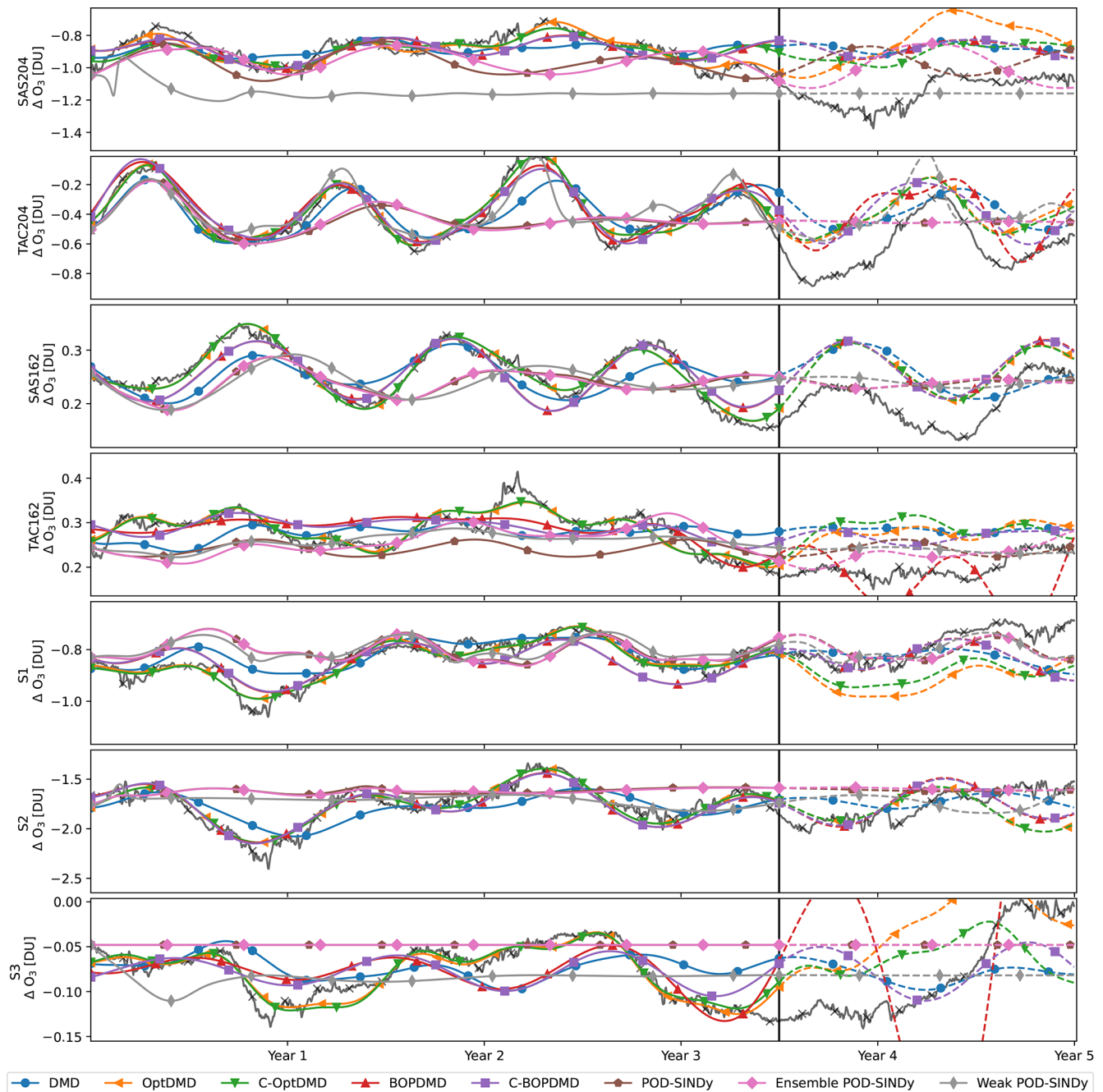
Figure 7. Reconstruction and forecast of the change in global column ozone in DU over time for all datasets and methods. The vertical black line denotes the change from the reconstruction to forecasting domains, solid lines are reconstructions and dashed lines mark forecasts of future behaviour.
