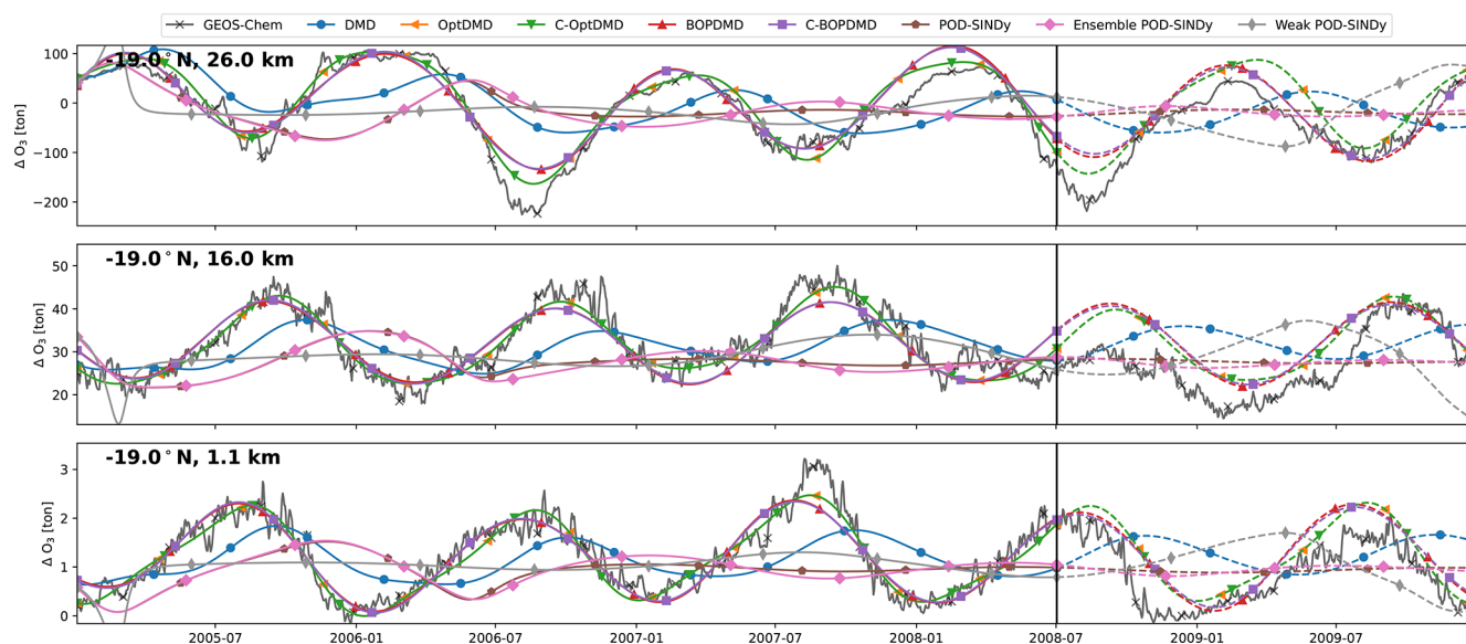
Figure C7. Same as Fig. C3, but for the S2 dataset.
