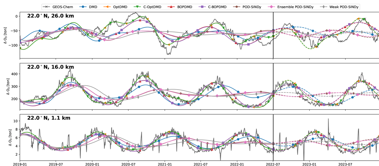
Figure C4. Same as Fig. C3, but for the SAS162 dataset.
