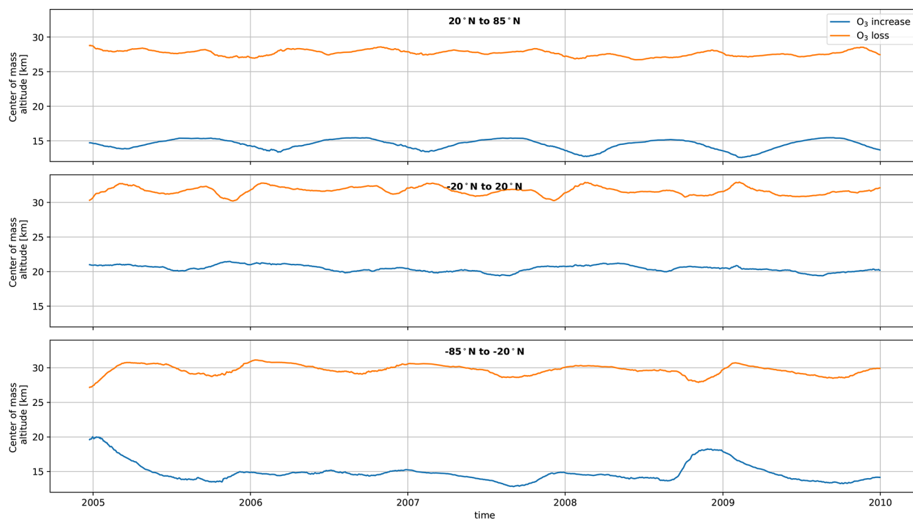
Figure C1. Altitude of the center of mass of the ozone response in the TAC204 dataset over time, calculated through a weighted average of the grid cells. Top row shows the northern hemisphere (20 to 85° N), the middle shows the tropics (−20 to 20° N), and the bottom row shows the southern hemisphere (−85 to −20° N).
