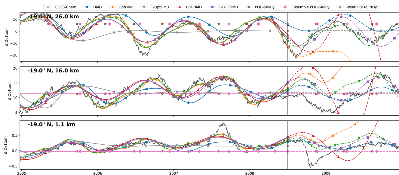
Figure C8. Same as Fig. C3, but for the S3 dataset.
