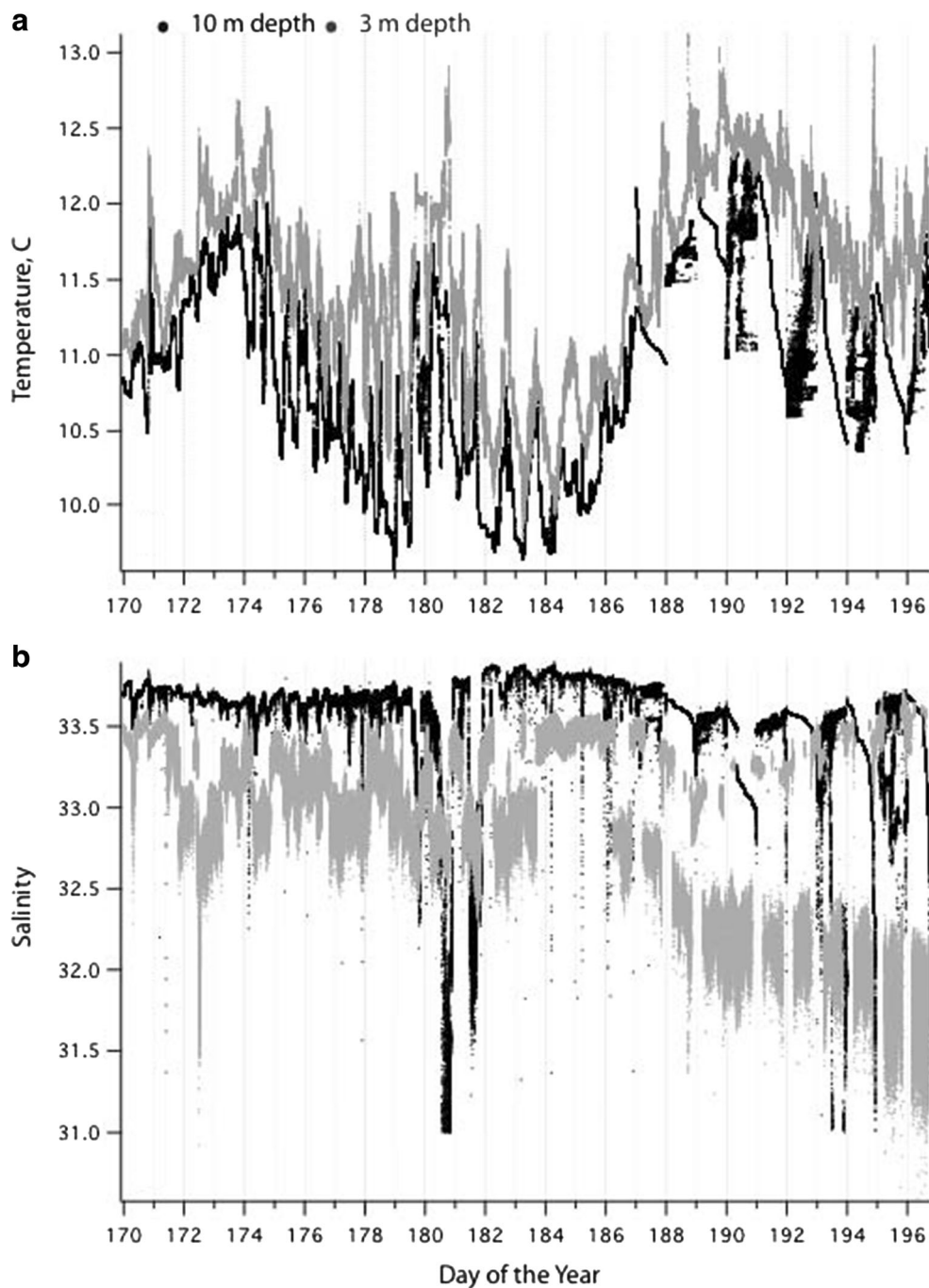
Fig. 11 Time series plots of a temperature and b salinity collected 125 m offshore at Carmel River State Beach. There were two CTDs: one at 10 m depth ( black dots ) and the other at 3 m depth ( gray dots )
