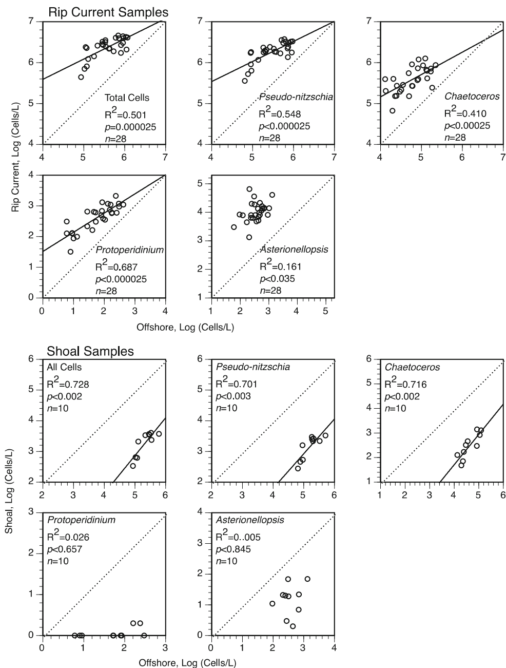
Fig. 6 Log of the concentrations of phytoplankton (all cells; the most abundant taxa, e.g., Pseudo-nitzschia and Chaetoceros ; all dinoflagellates; and the only surf zone diatom, Asterionellopsis ) collected offshore plotted against the log of the concentrations in the bathymetric rip current ( upper set of graphs ) and over the shoal adjacent to the rip current ( lower set of graphs ) at Sand City, California. The dotted lines indicate one-to-one relationships between phytoplankton concentrations. The solid lines and statistical results indicate significant regressions between the variables. Where solid lines are absent, the regressions were not significant. Significance levels were modified with a Holm-Bonferroni correction
