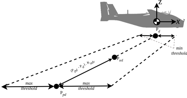
Figure 7: Setpoint generation.
