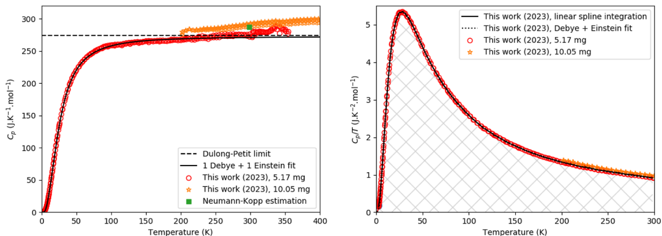
Figure 3. Experimentally measured heat capacity of Cs 4 PbI 6 as measured in this work and compared with the Dulong-Petit law, the Neumann–Kopp estimation at 298.15 K, and a fit of 1 Debye and 1 Einstein function as plotted in C_p vs T (Left) and C_p/T vs T (Right). The marked area in the right figure corresponds to the entropy as determined using linear spline (see main text).
