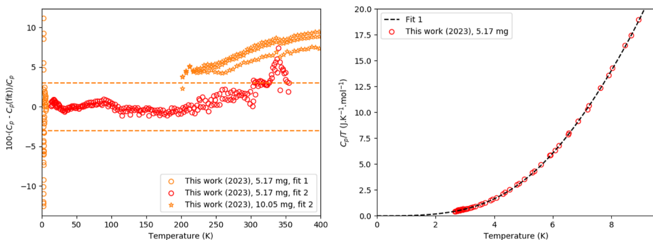
Figure 4. Left: Relative difference between experimentally measured heat capacity of Cs 4 PbI 6 as measured in this work and fitting functions. Fit 1 is a fit by a polynomial equation at low temperature (eq 4); Fit 2 is the fit of one Debye and 1 Einstein function. The dashed orange lines are a guide to the eye and are drawn at a 3% deviation from the fit. Right: the low-temperature part, using eq 4 (fit 1).
