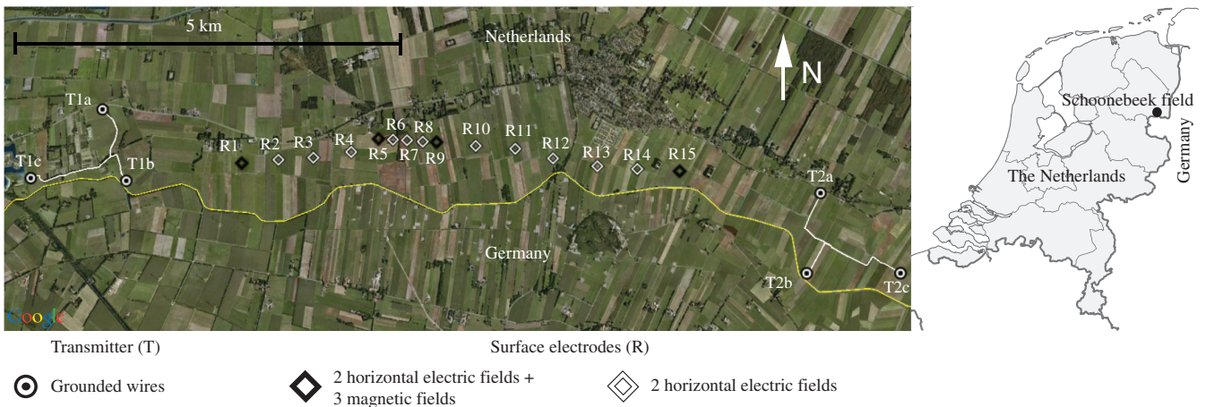
Figure 10. Location of field survey and detailed survey layout. Two transmitters are located west and east of the receiver line, respectively.
