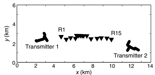
Figure 1. Source and receiver positions used for synthetic studies and field example.
