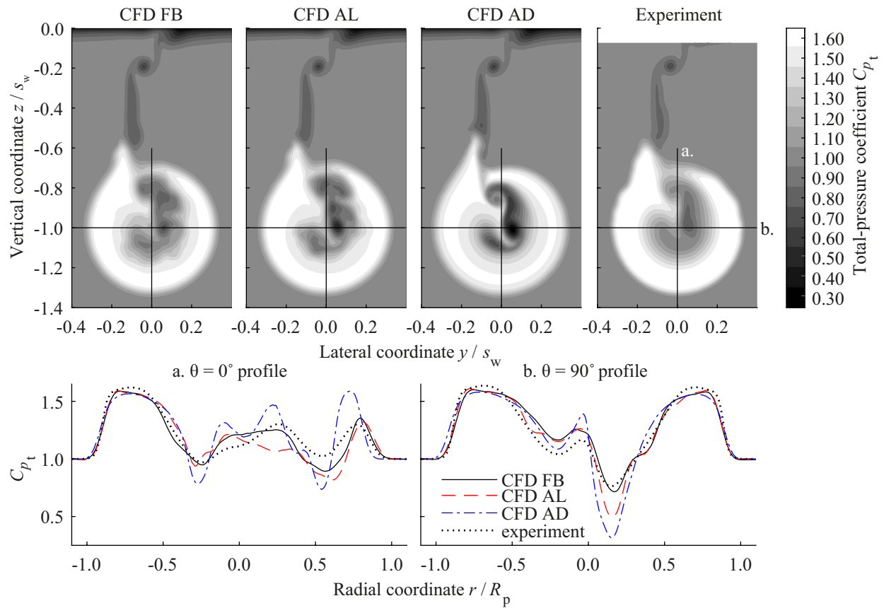
Fig. 18 Time-averaged total-pressure coefficient at the survey plane, \delta_f = +10^\circ .
