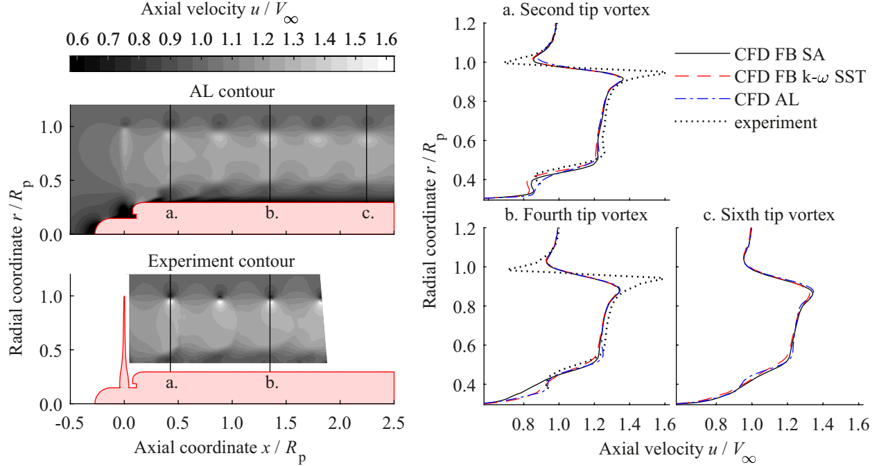
Fig. 12 Axial-radial contour plots through the blade pitch axis showing the phase-locked axial velocity for the actuator-line model and experiment. Radial profiles provide comparison with the full-blade model.
