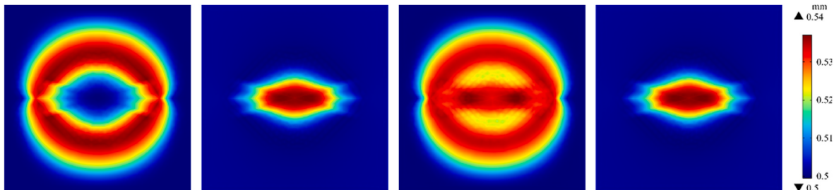
Fig. 17. Fracture aperture distributions of fracture F after 5 years under TH, THM, THM + C and THMC models (left to right).
