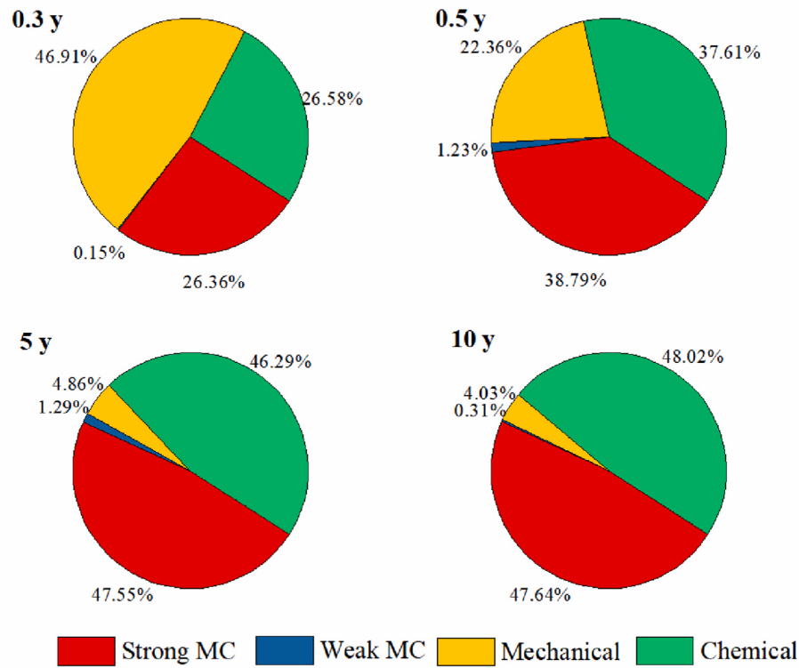
Fig. 20. Relative magnitude of mechanical, chemical, strong MC coupling and weak MC coupling over 0.3, 0.5, 5 and 10 years.
