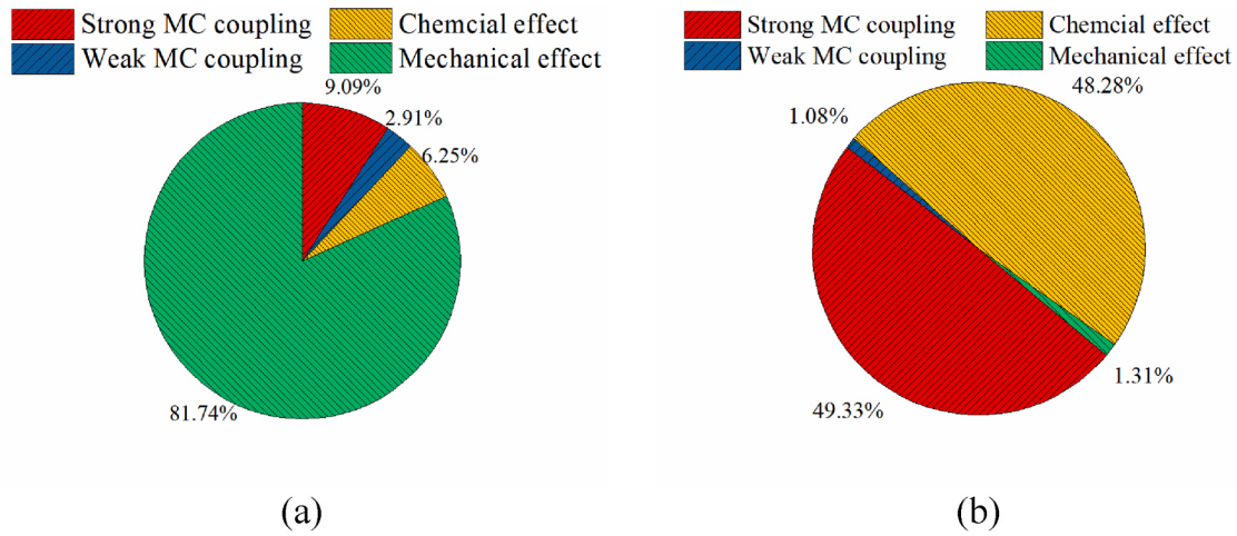
Fig. 23. The relative intensity for positions (a) point A around the injection well and (b) point C far from the injection well.
