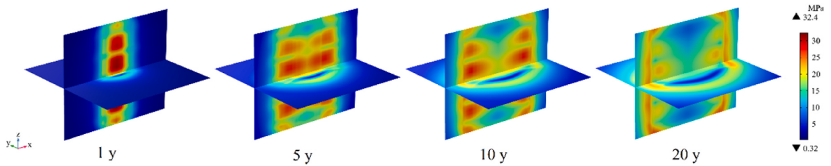
Fig. 10. Reservoir Mises stress distribution after 1, 5, 10 and 20 years.
