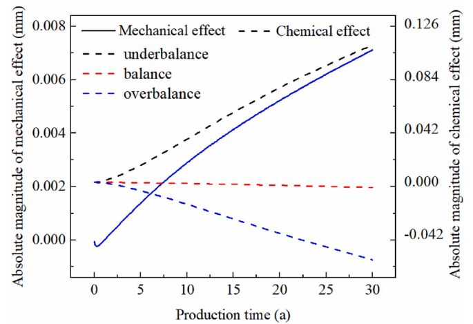
Fig. 25. The influence of injection concentration on the absolute magnitudes of mechanical and chemical effects.
