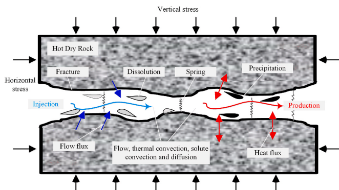
Fig. 1. Multi-physics processes in the fracture during EGS production (Song, G. et al., 2022b).
