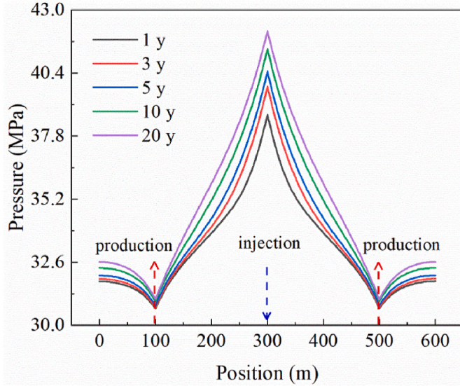
Fig. 9. Pressure distribution along the line P_1P_2 between wells after 1, 3, 5, 10 and 20 years.
