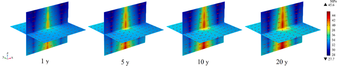
Fig. 8. Reservoir pressure distribution after 1, 5, 10 and 20 years.
