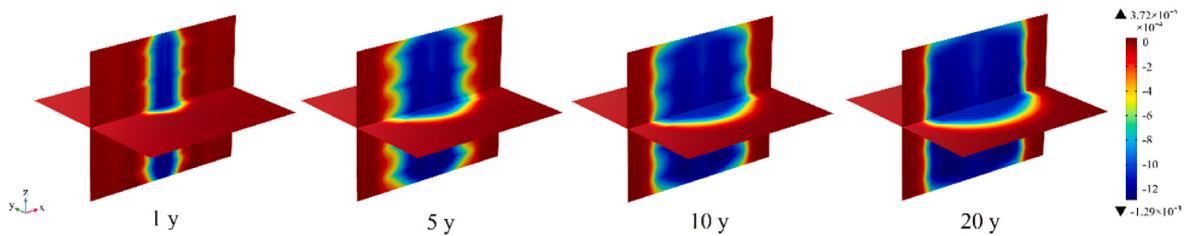
Fig. 11. Reservoir volumetric strain distribution after 1, 5, 10 and 20 years.
