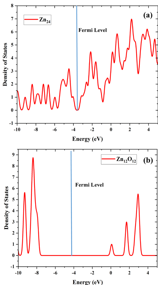
Figure 7. TDOS plots for the isolated (a) \text{Zn}_{24} and (b) \text{Zn}_{12}\text{O}_{12} clusters calculated at the TPSSh/LAN12Dz level of theory.
