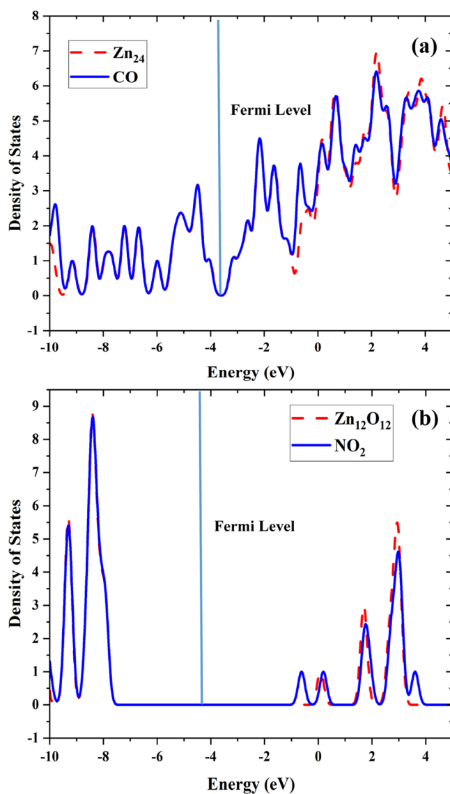
Figure 8. TDOS plots for (a) \text{CO}/\text{Zn}_{24} and (b) \text{NO}_2/\text{Zn}_{12}\text{O}_{12} systems calculated at the TPSSh/LAN12Dz level of theory.
