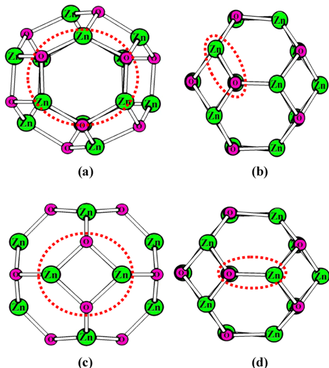
Figure 2. Different adsorption sites (indicated by the regions within the dashed circles) that can be identified in the \text{Zn}_{12}\text{O}_{12} cluster are (a) in the space surrounded by the hexagonal ring, (b) the bond between the hexagonal ring and the quadrilateral ring, (c) inside the space surrounded by the quadrilateral ring, and (d) the bond between two hexagonal rings.
