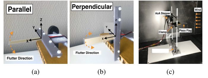
Fig. 3: (a) Parallel (in-plane) configuration of inverted flag. (b) Perpendicular (out of plane) configuration of inverted flag. (c) Constructed test rig.
