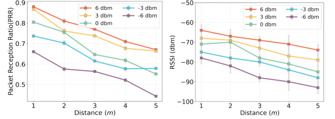
Fig. 16: Packet reception ratio (PRR) and RSSI of for varying distance and transmission power.
