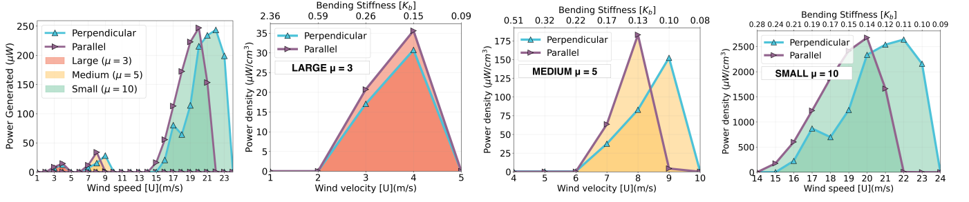
Fig. 5: Evaluation of harvested energy by all flags for \alpha = 0 (left) and interpreting the power density variations with bending stiffness for \mu = 3 , \mu = 5 and \mu = 10 .
