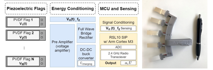
Fig. 11: Hermes system block diagram and fabricated sensor.
