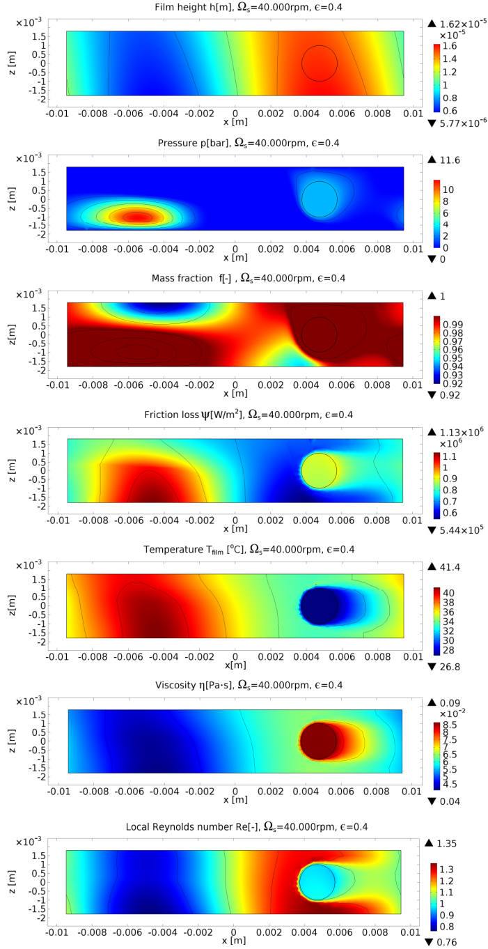
Figure 3.18: Contour plots of the bearing fluid domain representing its state at a rotation speed of \Omega_s = 40,000\text{rpm} and an eccentricity ratio of 0.4 . The data is taken from a run-up simulation of the coupled rotor-bearing system. The absence of symmetry over the axis z=0 is due to shaft tilting.
