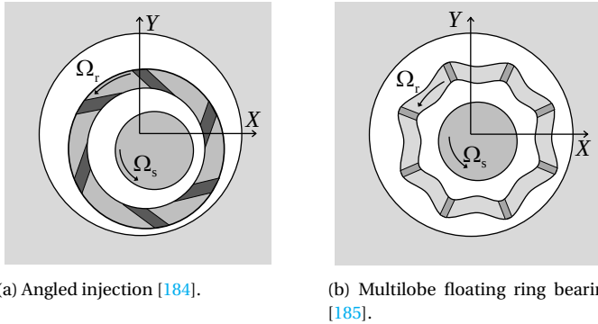
Figure 2.12: Alternative bearing geometries.
