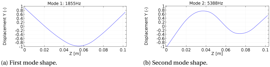
Figure 5.5: Modal analysis of the turbocharger rotor based on a FEM model using beam and disk elements. The compressor wheel is mounted to the left hand side of the rotor, the turbine wheel to the right hand side.
