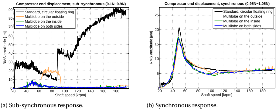
Figure 5.26: Simulation data: shaft displacement as a function of multilobe configuration.
