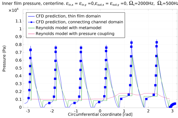
(a) Inner film pressure
