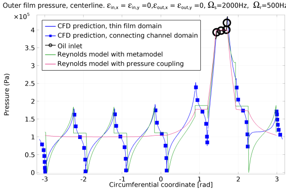
(b) Outer film pressure
