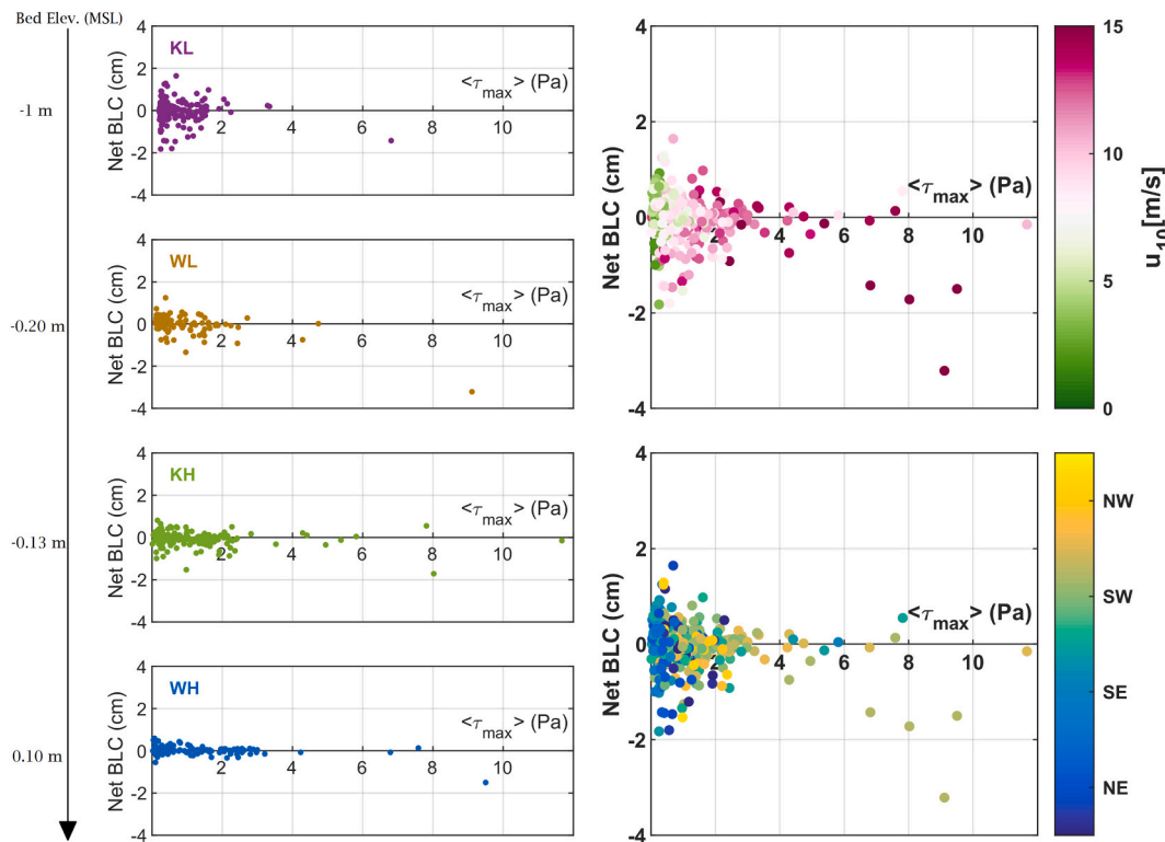
Fig. 3. Net bed level changes (BLC) per tidal cycle (one marker represents one tidal cycle) as a function of tide-averaged maximum bed shear stress at each site (left panels). The right panels include the net BLC measured at all sites. Upper right panel: BLC as a function of tide-averaged maximum bed shear stress and wind speed; lower right panel: BLC as a function of tide-averaged maximum bed shear stress and wind direction. The combined wave-current bed shear stress has been computed using (Soulsby, 1995)'s method.
