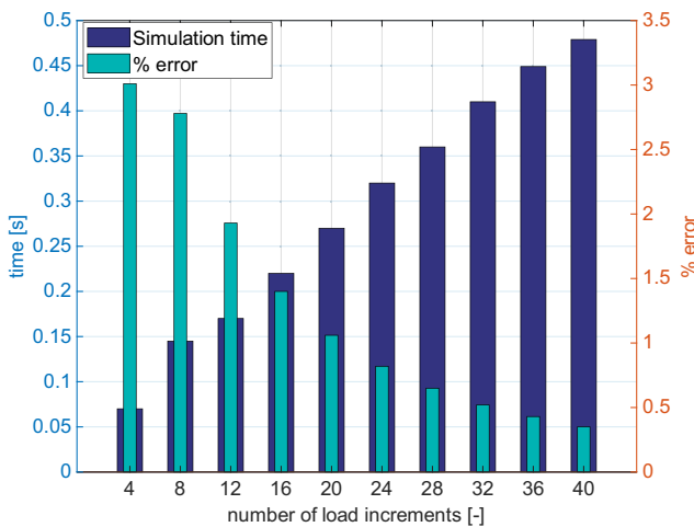
Fig. 6 Depiction of the influence of the number of load intervals on the simulation time (in seconds) and accuracy of analysis (percent error) at a load of 700 \text{ N/m} .
