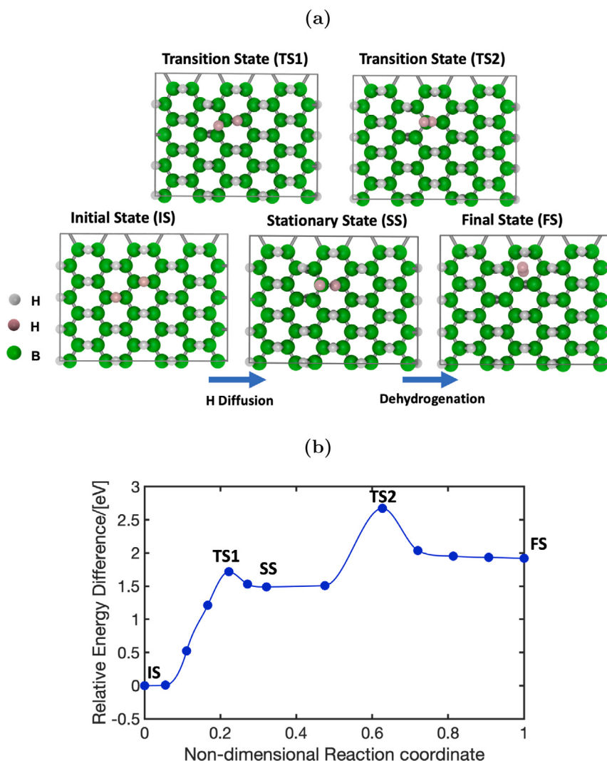
Fig. 3. (a) The structural configurations corresponding to the minimum energy pathway for a single H 2 release on 2D BH. The H atoms that are undergoing reaction are shown in pink while the rest of H-atoms are colored gray. To reach the final state from the initial state, one of the H-atoms initially hops to a neighboring boron atom (stationary state) and consequently the two H-atoms react to form a H 2 molecule. The transition states for each of the two processes are shown. (b) The minimum energy pathway for a single H 2 release for the path depicted in (a) as a function of a non-dimensional reaction coordinate. The TS1, SS, TS2, and FS states have a energy difference of 1.72, 1.53, 2.68, and 1.92 eV with respect to the IS state, respectively. The lines connecting the NEB images (constructed using forced-based cubic splines) are to guide the eye.
