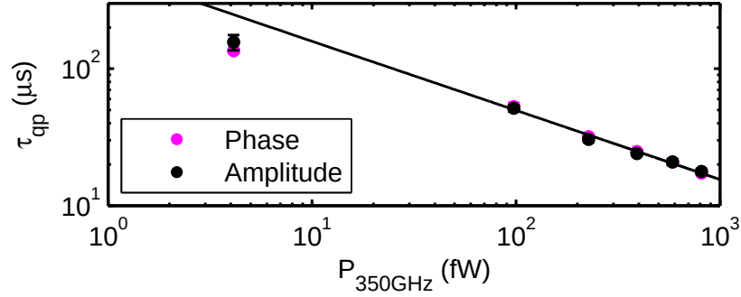
Figure 7.3: The quasiparticle lifetime, determined from the phase (magenta) and amplitude (black) noise roll-off, as a function of optical power absorbed by the MKID, P_{350\text{GHz}} . The Lorentzian fit gives a typically error of 5% in the estimated lifetime. As a result, error bars are usually smaller than the symbol size. A fit to the measured lifetimes for P_{350\text{GHz}} > 100 fW shows that \tau_{qp} \propto P_{350\text{GHz}}^{-0.50 \pm 0.02} .
