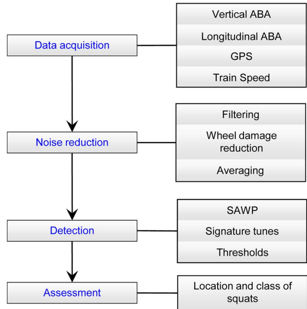
Fig. 9. Detection procedure.
