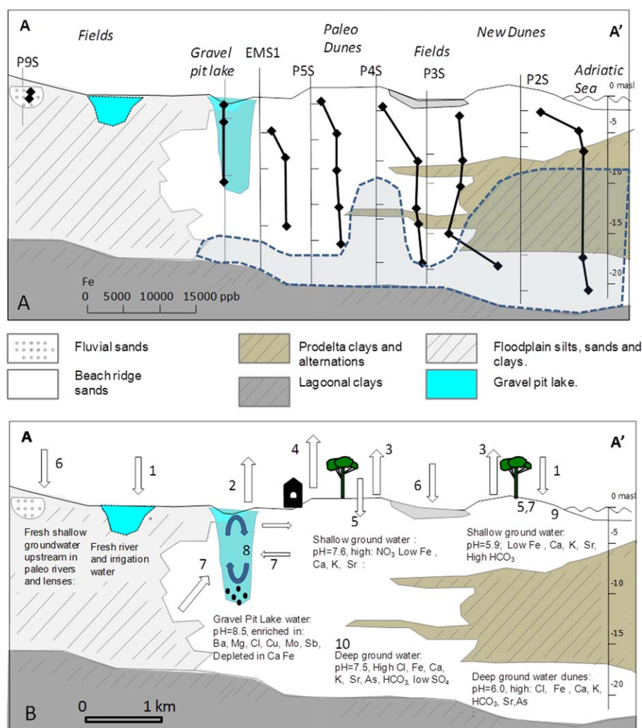
Fig. 3. (a) Profile through the aquifer and across gravel pit lake EMS from well P9S to the Adriatic Sea. Vertical concentration profiles of Fe are shown in interconnected bold black dots along well trace to illustrate the increase in concentration of Fe as many other elements towards the Adriatic Sea, depletion of shallow groundwater with respect to deeper groundwater and typically a relative depletion or enrichment in the gravel pit lake. Location of wells and sampling points are shown, (b) summary of hydrochemistry and hydrochemical processes occurring in and around the coastal gravel pit lake. Arrows indicate direction of water flow. Numbers correspond to the following processes: (1) precipitation and natural recharge of the gravel pit lake and aquifer, land upstream and dunes downstream. (2) Evaporation from lake surface. (3) Transpiration by pine trees. (4) Drainage of water seawards. (5) Groundwater table fluctuation exposing sediments to oxygen. (6) Fertilization of soil brings \text{PO}_4 and \text{NO}_3 in groundwater. (7) Redox reactions involving Fe(hydr)oxides or Pyrite, then Fe, and As (among others) are released into groundwater. (8) Groundwater exfiltrates into lake. (9) Groundwater rich in dissolved metals comes into contact with basic lake water enriched in oxygen; metal oxides and \text{CaCO}_3 precipitate. (10) Sulfate reduction.
