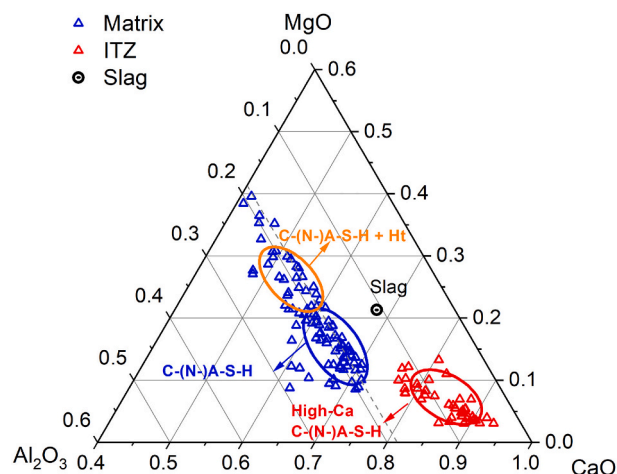
Fig. 11. CaO-Al 2 O 3 -MgO ternary diagram of EDX spot analysis in the ITZ.
