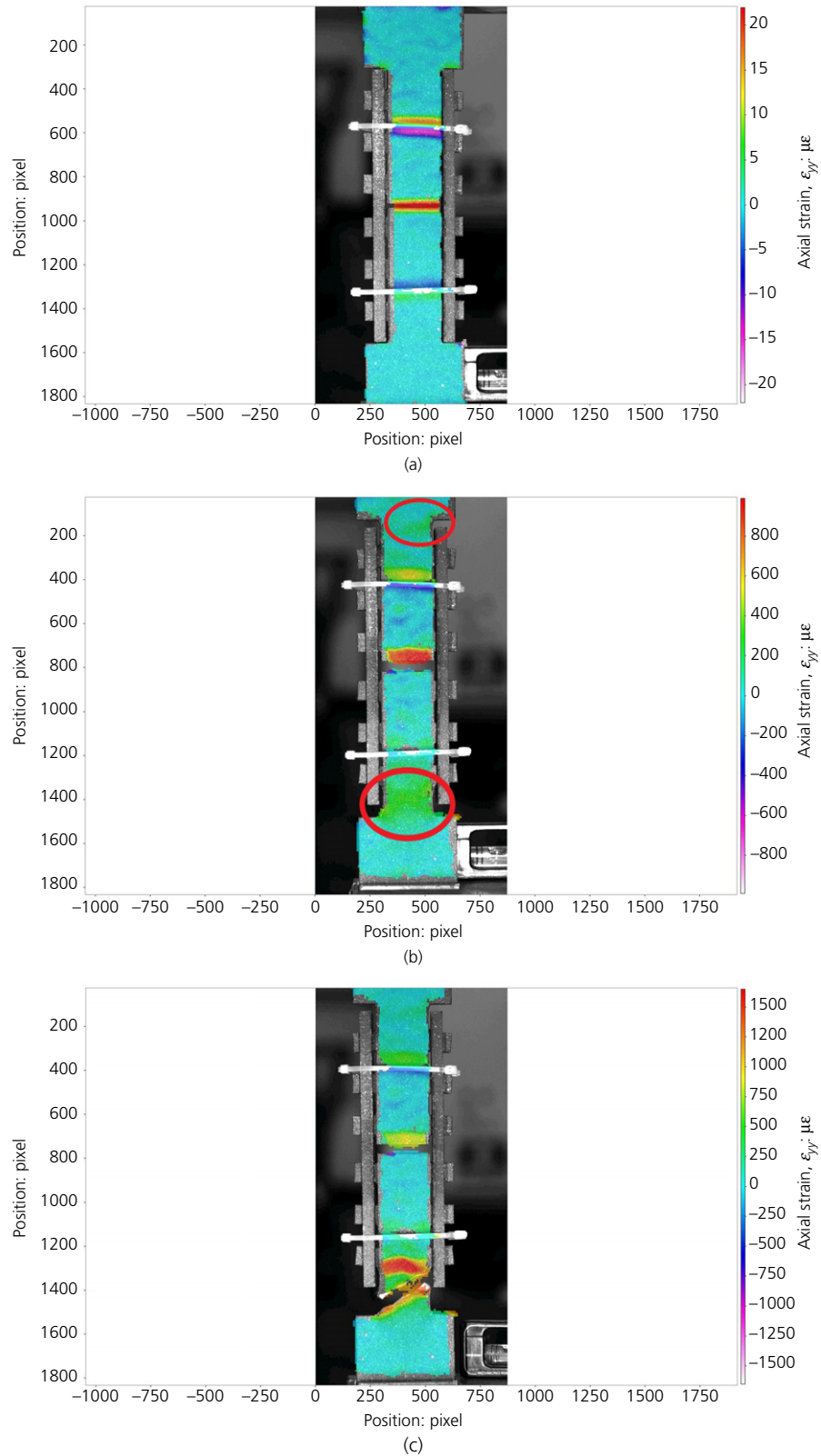
Figure 10. Strain contours from DIC: (a) initial stage; (b) prior to failure; (c) at failure. A full-colour version of this figure can be found on the ICE Virtual Library ( www.icevirtuallibrary.com )
