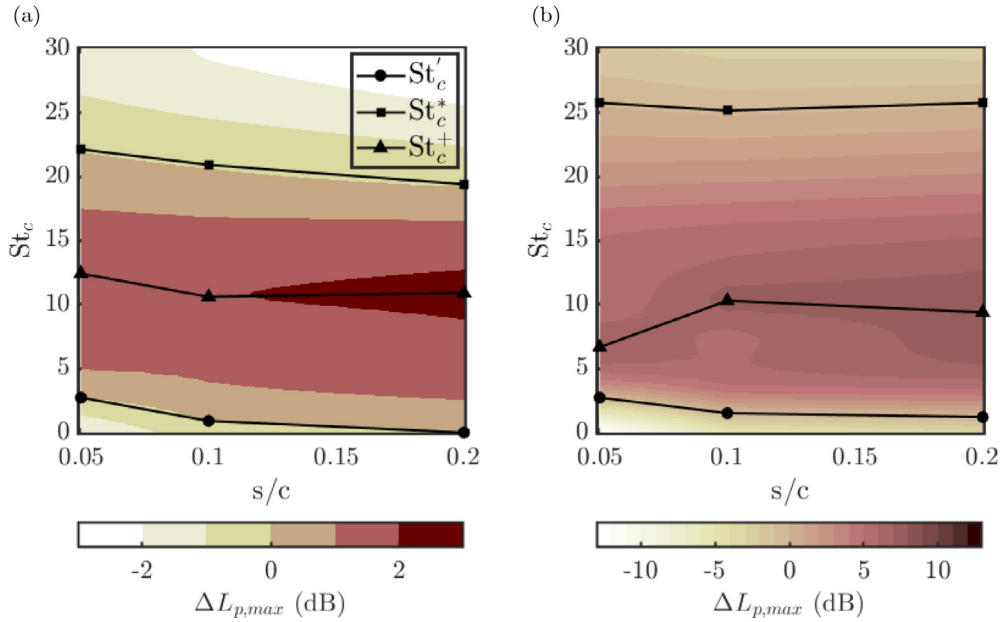
Fig. 21. Change in maximum noise attenuation \Delta L_{p, \text{max}} with permeable chordwise length s/c and chord-based Strouhal number St_c for perforated inserts with l_h = 5 (a) and 2 mm (b) at \alpha = 0.2 degrees.
