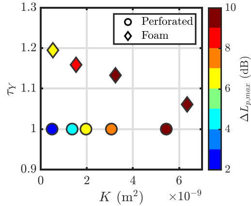
Fig. 18. Maximum noise attenuation \Delta L_{p,max} as a function of K and \tau_Y for \alpha = 0.2 deg.
