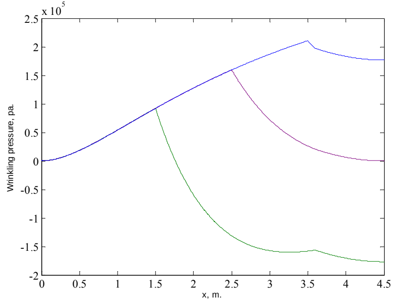
Figure 11. Minimum internal pressures as a function of x for three different positions of the bridle line. b_2 = 1\text{m} in blue, b_2 = 2\text{m} in purple and b_2 = 3\text{m} in green.
