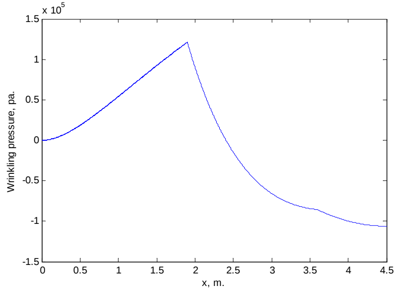
Figure 12. Minimum internal pressures as a function of x for b_2 = 2.6\text{m} .
