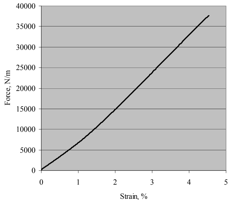
Figure 6. Test result of the unbonded laminate.
