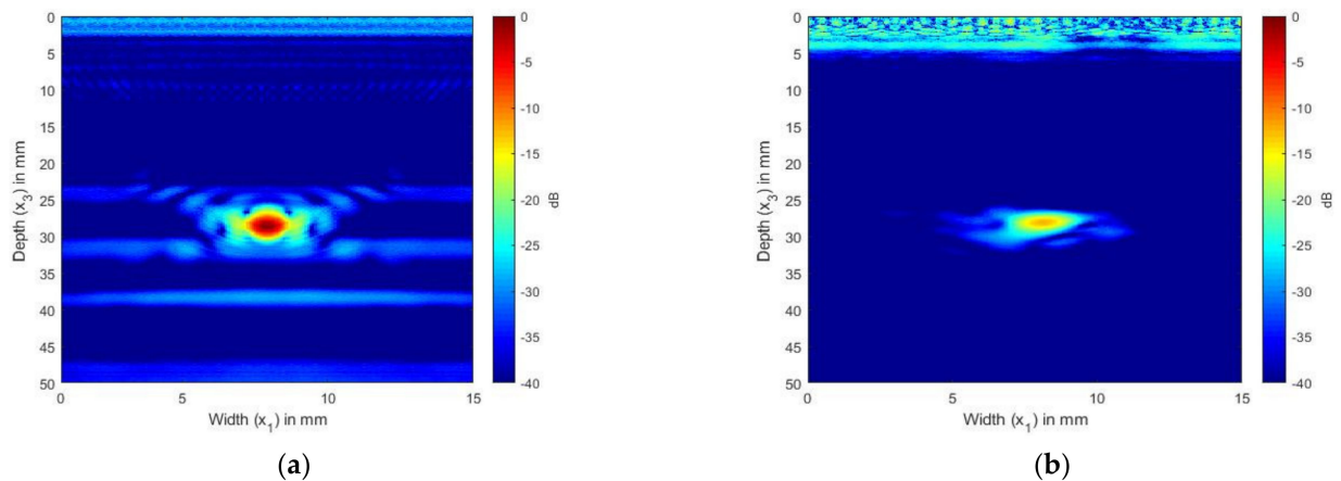
Figure 4. (a) TFM image of simulated SDH FMC signals in aluminum using the 2.25 MHz array; (b) TFM image of experimental SDH FMC signals in aluminum using the 2.25 MHz array.
