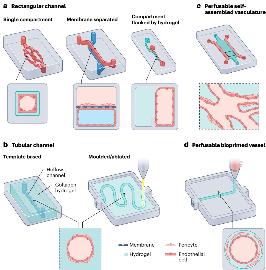
Fig. 2 | Design principles of MPSs of the human vasculature. a , Left, a single patterned channel, usually made with PDMS or an agarose gelatin hydrogel, is widely used for monocultures of endothelial cells. Middle, two aligned channels separated by a porous membrane. Unidirectional pressure-driven fluid flow can be introduced in both channels. The device is made of PDMS and coated with a thin hydrogel layer. Cells can be cultured in both channels. The top channel is usually seeded with tissue-specific cell types (such as astrocytes, neurons, lung epithelium or intestinal epithelium) and the bottom channel is seeded with endothelial cells. Right, a two-channel device designed for use with gravitational bidirectional flow. One channel is used to seed endothelial cells and is flanked by a hydrogel-filled channel separated using a phase guide. Tissue-specific cells can be seeded in the hydrogel channel. b , Left, tubular channels that use
