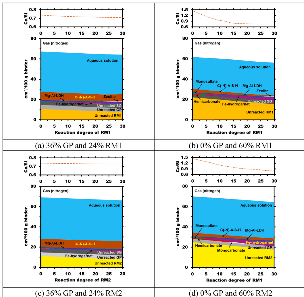
Fig. 15. Thermodynamic simulation of four typical RM-incorporated reaction systems and the Ca/Si ratio of the predicted C(N)-A-S-H assuming different reaction degrees of RM (0 %–30 %). The reactivities of GP and SG were assumed to be 50 %.
