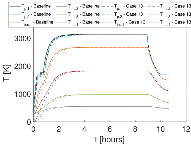
Fig. 10. Simulation temperature profile results of the Baseline case and Case 13 versus time for one orbit assuming a 640 min orbital period and a 104 min eclipse.
