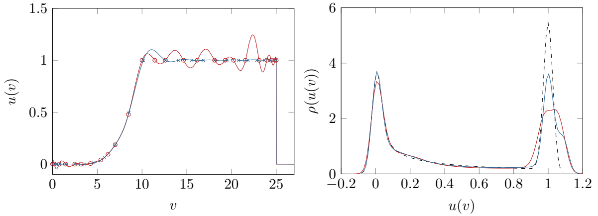
Figure 3: The interpolated P - v curve and the resulting distribution of u(v) using 25 nodes (shown in the left figure) for the propagation problem with \zeta = 0 (in red) and \zeta = 1/3 (in blue). The dashed distribution is the exact distribution.
