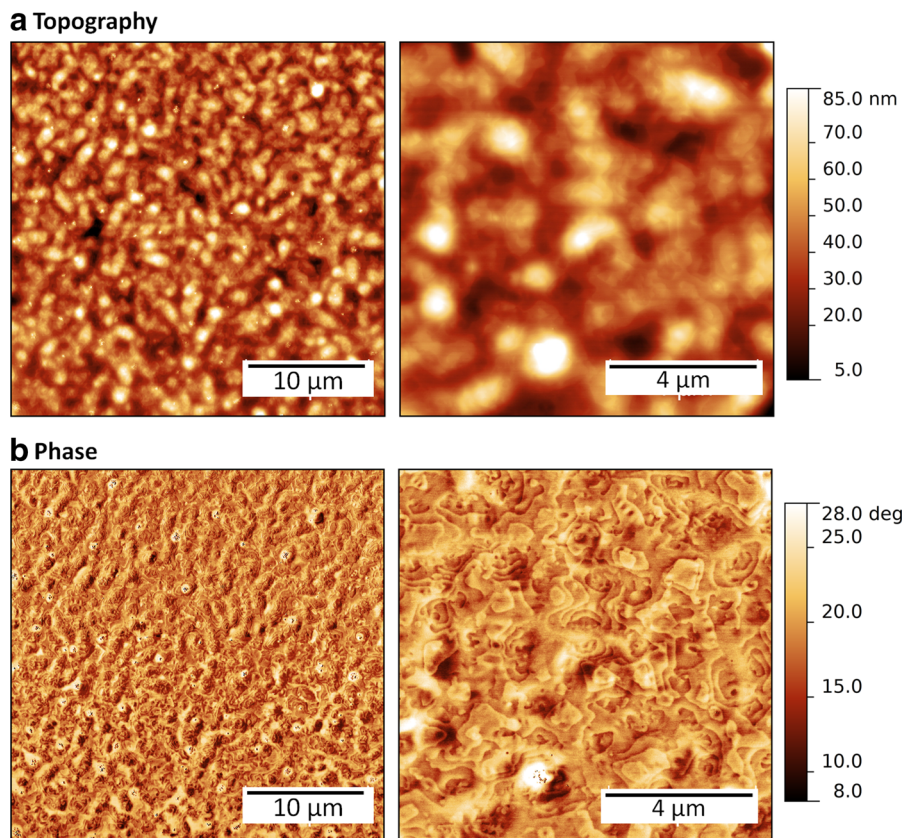
Fig. 7 Microstructure of 30 wt% asphaltene sample: a AFM topography and b AFM phase images of both 30 \times 30 and 10 \times 10 \mu\text{m}^2
