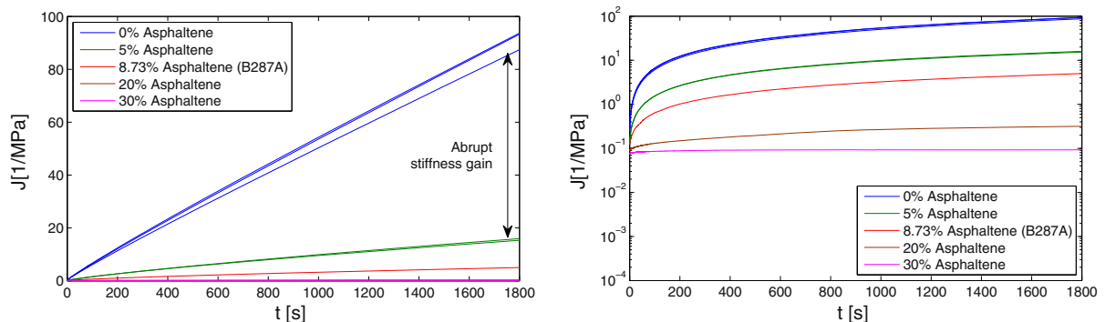
Fig. 3 Creep response of bitumen samples from CR tests at +5^\circ\text{C}
