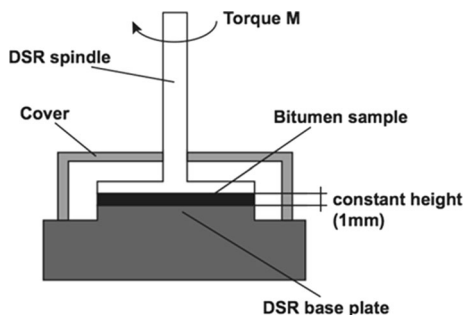
Fig. 2 Creep-recovery test using DSR experimental equipment
