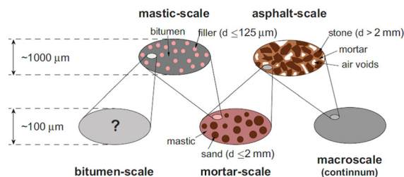
Fig. 1 Multi-scale model of hot mix asphalt according to [30–34]—microstructure of bitumen not yet considered
