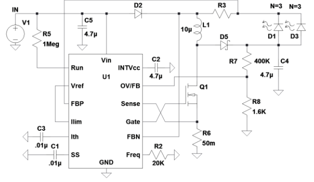
Fig.1 The Electrolytic Capacitor-Free Buck-Boost LED Driver
