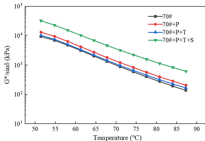
Fig. 6. Rut factor ( G = \sin \delta ).
