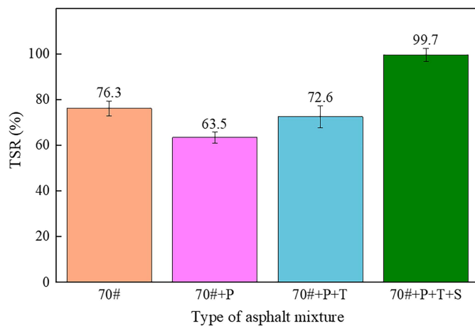
Fig. 14. Freeze–thaw split test data.
