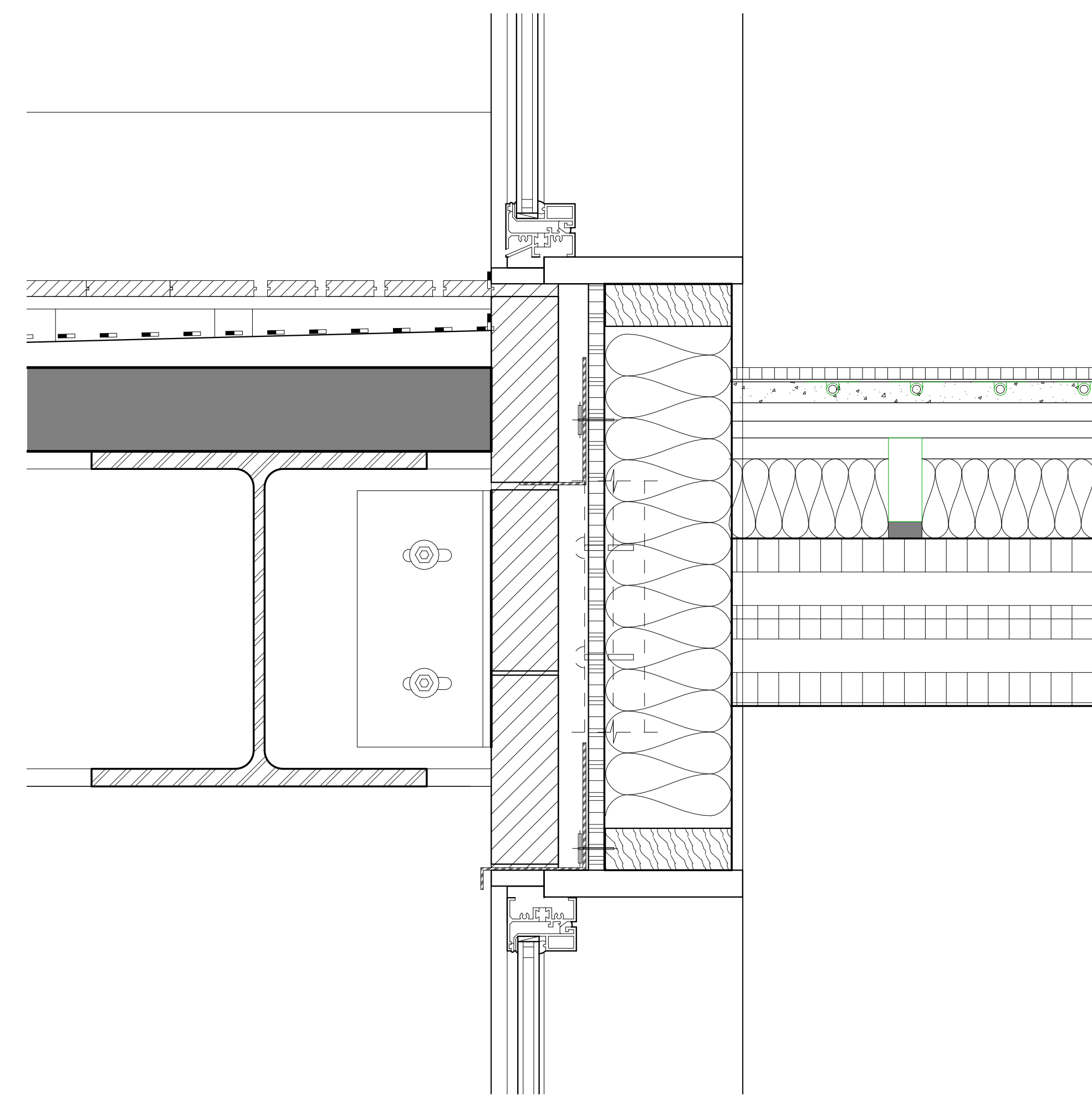
South Residential Facade Section / Elevation Studio Units and Balcony 1:20
