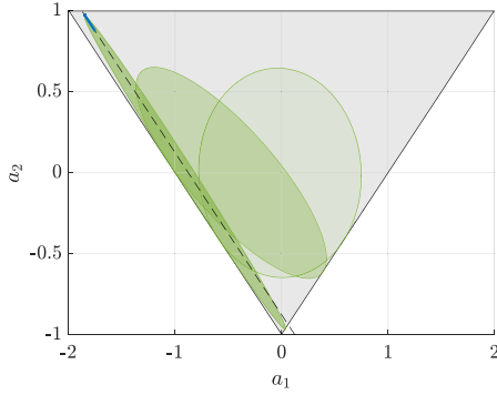
Fig. 3. Coefficient set \mathcal{A}_P = \{A = [a_1 \ a_2] \mid (F - GA)^\top P(F - GA) - P < 0\} , i.e., the set of unstructured coefficients for which P proves stability at step 1 (○), 10 (●) and 23 (●) of the optimization. At every step, the intersection of \mathcal{A}_P with the affine structure set (---) is not empty, i.e., the structured coefficient set \tilde{\mathcal{A}}_P = \{\tilde{A} = d \mid (F - G(h + \tilde{A}H))^\top P(F - G(h + \tilde{A}H)) - P < 0\} is not empty. During identification, P is optimized in such a way that the true system with A(\rho) as in (18) (—) is contained in \mathcal{A}_P . Each \mathcal{A}_P is contained within \mathcal{A} (▽), i.e., the set of unstructured coefficients that result in a stable system in the LTI case.
