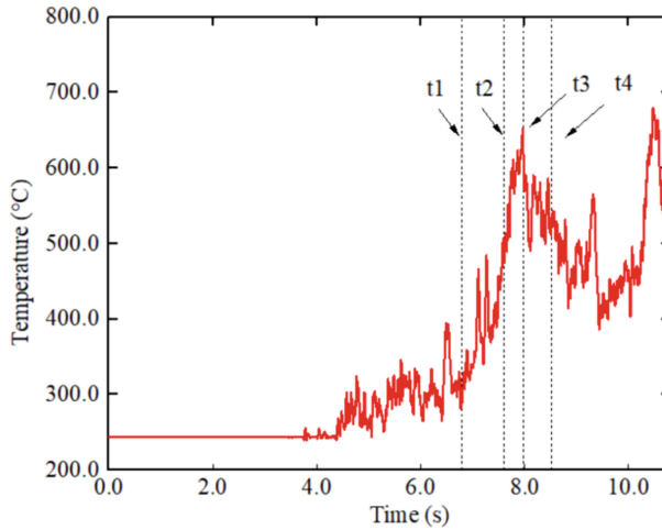
Fig. 3. The maximum temperature in the ROI varying with time
