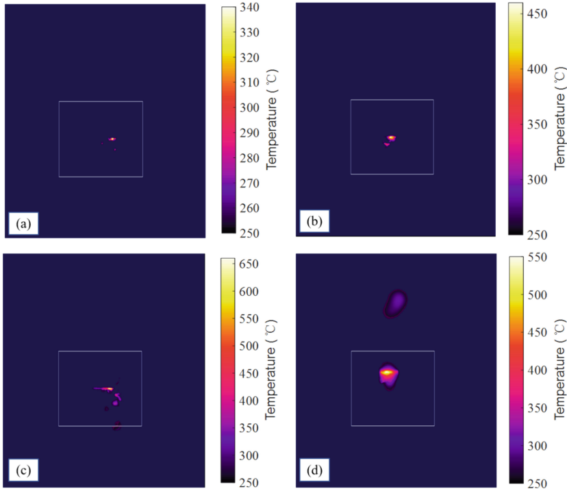
Fig. 4. Thermal images during the measurement described by the temperature at different slip ratios (denoted by s ): (a) s = 8.3\% , (b) s = 15.9\% , (c) s = 20.4\% , (d) s = 41.4\%
