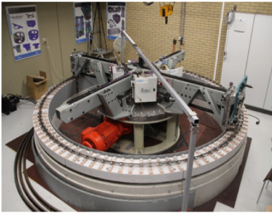
(a) An overview of the test rig
