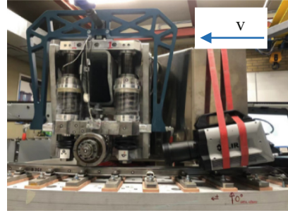
(b) The high-speed thermal camera mounted on the test rig
