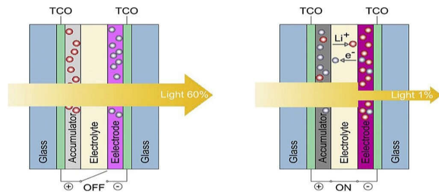
Figure 13. Schematic principle of operation of electrochromic glazing (retrieved from [13]).
