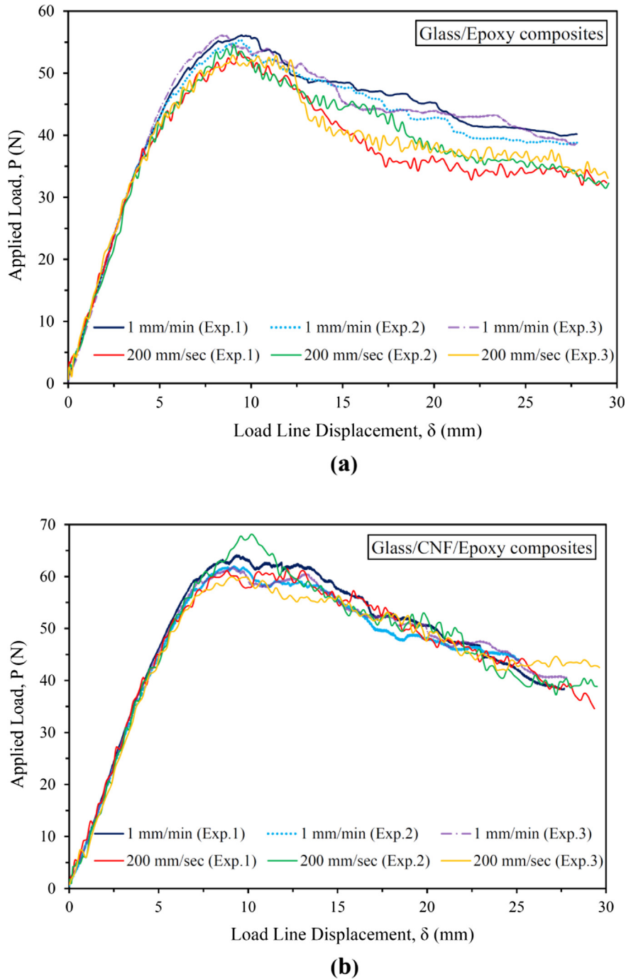
Fig. 5. Load-displacement curves for (a) glass/epoxy and (b) glass/CNF/epoxy composite specimens tested at quasi-static and 200 mm/sec loading rates.
