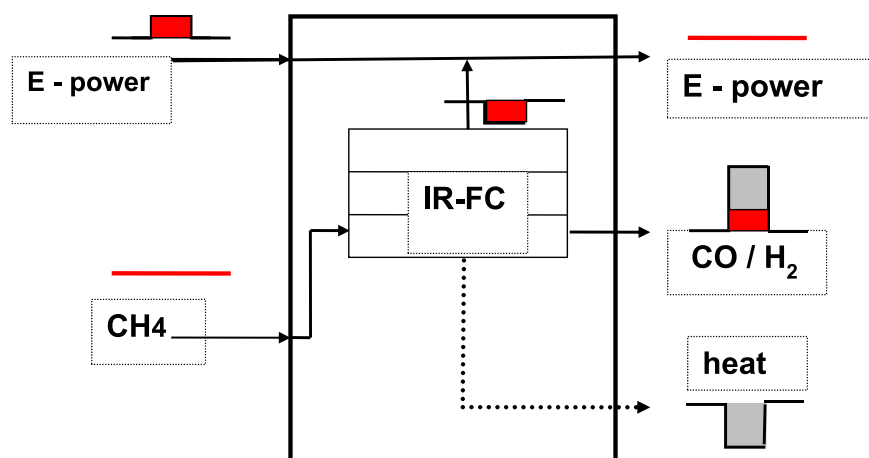
Fig. 4 – Superwind concept.
