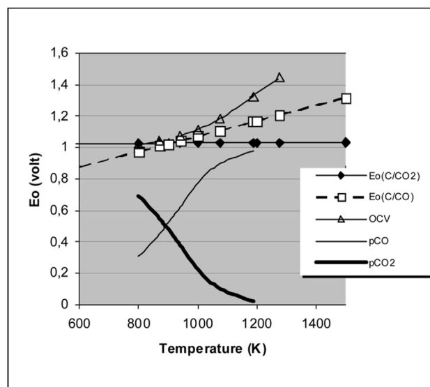
Fig. 2 – Standard potentials for the oxidation of carbon to CO and CO 2 and the Open Cell Voltage of a carbonate DCFC assuming p_{\text{CO}} + p_{\text{CO}_2} = 1 \text{ atm} at the anode and p_{\text{O}_2} = p_{\text{CO}_2} = 1 \text{ atm} [From Hemmes & Cassir [18]].
