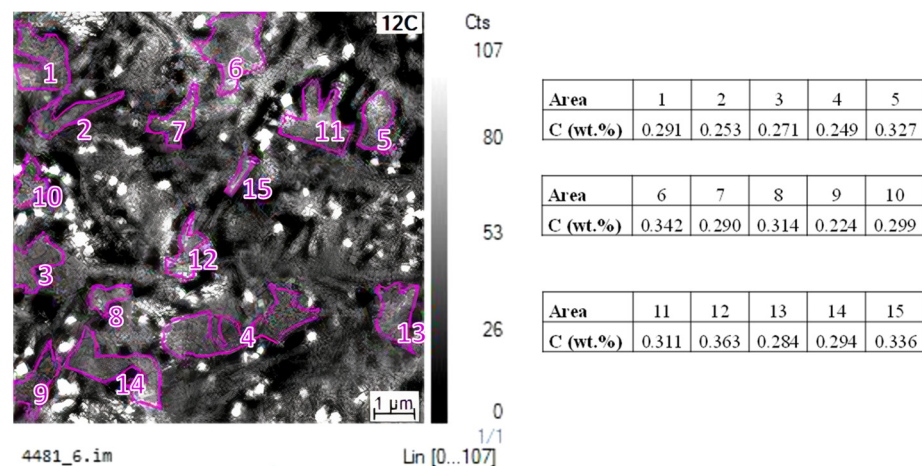
Figure 8. Example of one ^{12}\text{C} ion map (left side) and carbon content estimated in different areas of this zone (right side) in M-MnNi steel sample partition-treated at 650 °C during 300 s and in QT15 condition. The areas selected for carbon content analysis are surrounded in purple in the ^{12}\text{C} ion map.
