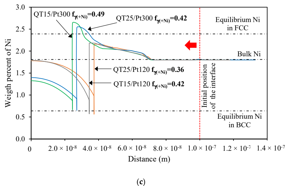
Figure 12. (a) Schematic of the system considered in DICTRA simulations; (b,c) DICTRA calculations of the Mn and Ni composition profiles, respectively, at the martensite (left)/austenite (right) system. The calculation was done considering the chemical composition of M-MnNi steel, 650 °C (PT), 120 s and 300 s (Pt) and 0.15 and 0.25 austenite volume fractions as initial conditions (QT15 and QT25, respectively).
