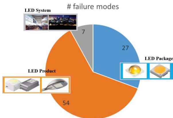
Figure 4: Pareto for the number of failure mode vs product type.
