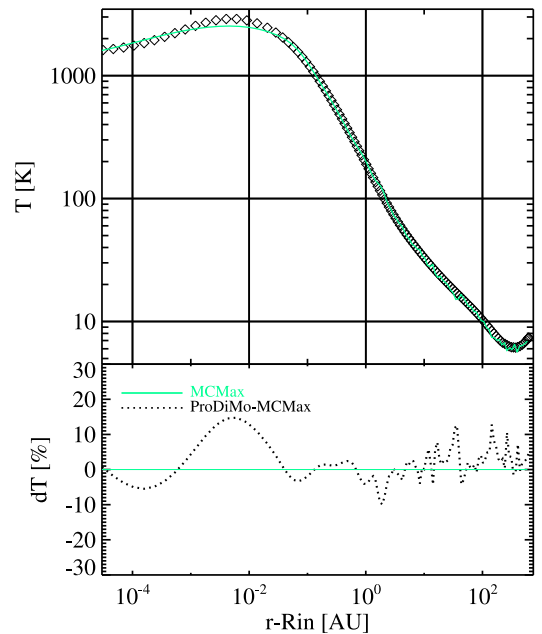
Fig. A.3: Midplane temperature T_{\text{dust}}(r, 0) as function of the log-distance from the inner rim. Again, the green line is the temperature profile calculated by MCMax, and the small black diamonds show the temperature values calculated by PRODiMo.
