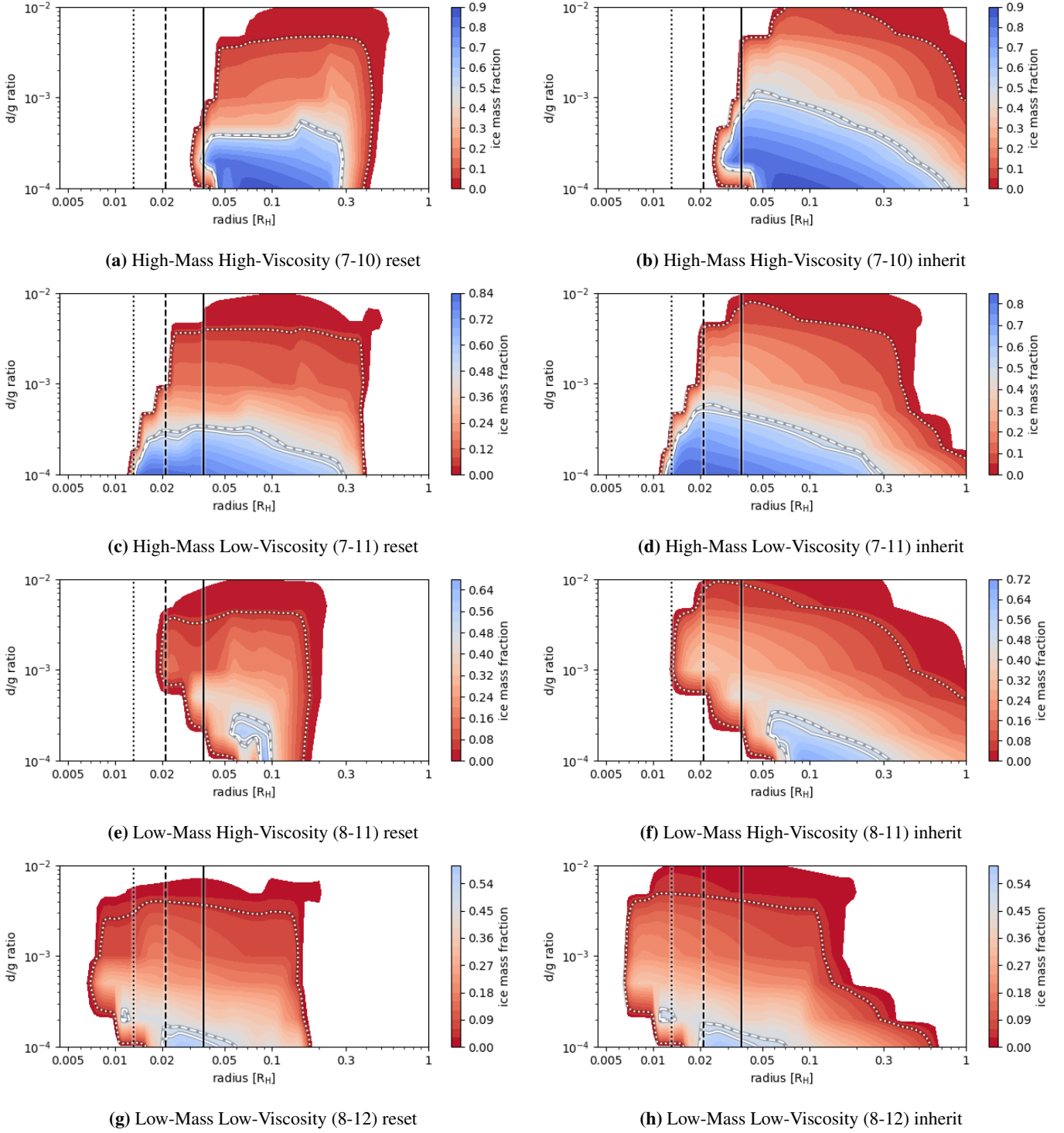
Fig. H.1: Midplane radial ice mass fraction f_{\text{ice}} of the dust-to-gas ratio parameter exploration for the chemically reset (left column) and chemically inherited (right column) reference CPDs. The black dotted, dashed, and solid lines indicate the radial position of Europa, Ganymede, and Callisto. The white dotted, dashed, and solid lines indicate where f_{\text{ice}} is equivalent to the estimated ice mass fraction of Europa (0.05), Ganymede (0.48), and Callisto (0.52).
