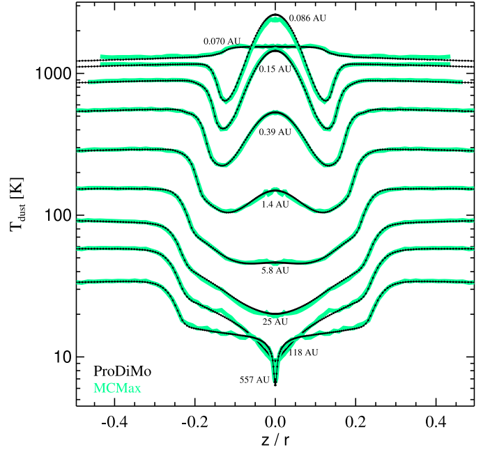
Fig. A.2: Benchmark test for a viscous circumstellar disk with a disk mass of 0.01 M_\odot and a mass accretion rate of \dot{M}_{\text{acc}} = 10^{-8} M_\odot/\text{yr} , see text. The green lines are temperature cuts at selected radii calculated by MCMax, the small wiggles are due to the Monte-Carlo noise. The black dots show the temperatures calculated by PRODiMo.
