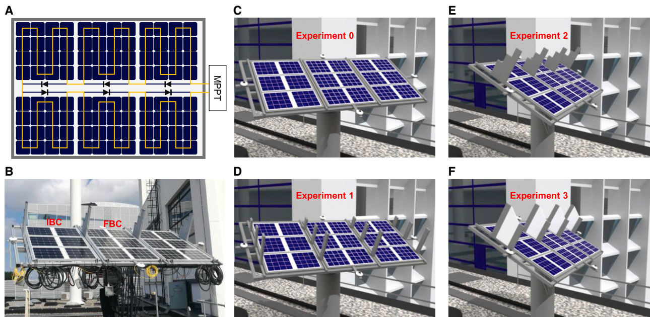
Figure 6. Experimental setup
