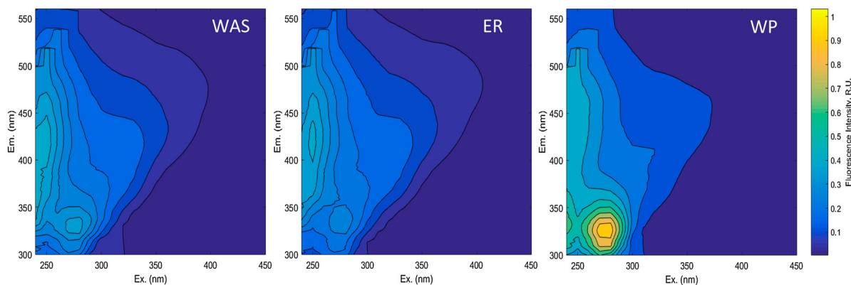
Figure 4. EEMS spectra of waste activated (WAS), endogenous respiration (ER) and worm predated (WP) sludges, respectively. Measurements were done in triplicate. The plots are representative off the triplicates. VS degradation percentages of the samples were the following: ER 16%; WP 24%.
