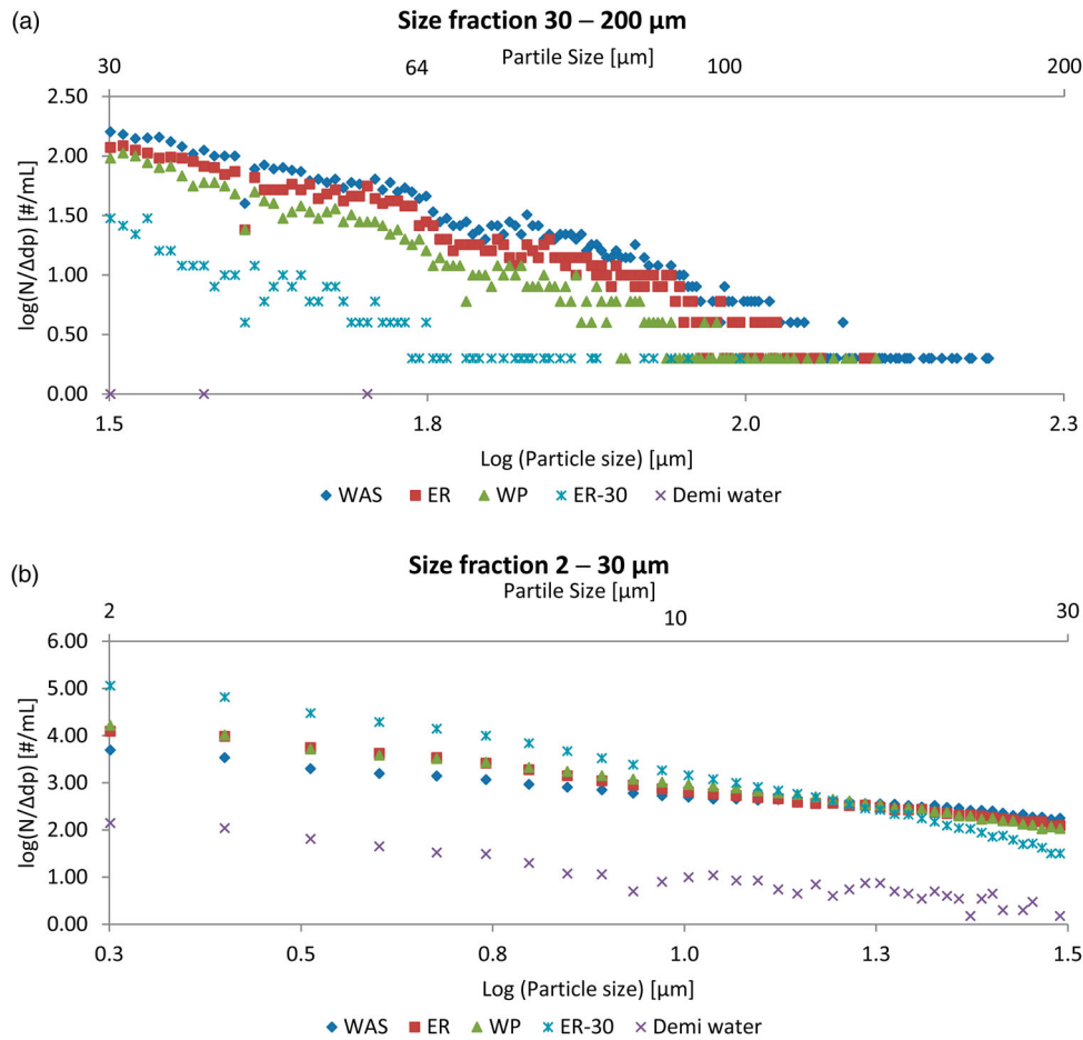
Figure 1. Normalized PSD of treated sludges, showing the averages of triplicate measurements. Graph split in two parts: (a) 30–200 μm; (b) 2–30 μm. Error bars are omitted for clarity. Horizontal line around 0.5 counts/mL*μm is due to low particle counts (1–2 counts/mL) in the measurements. The outlier at 1.6 μm* is probably due to a fault in the machine as it is consistent in all the measurements. Particles larger than 200 μm were not observed in the sludges. Batch VS reduction was for WP 42%, ER 18% and ER-30 29%. For visualization, the values plotted were not multiplied by the dilution factor.
