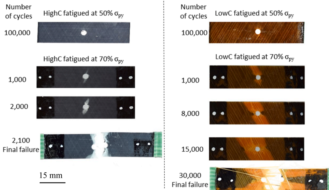
Fig. 11. (a) Typical damage mechanisms for the open-hole laminates fatigued at 50% of \sigma_{py} and 70% of \sigma_{py} .
