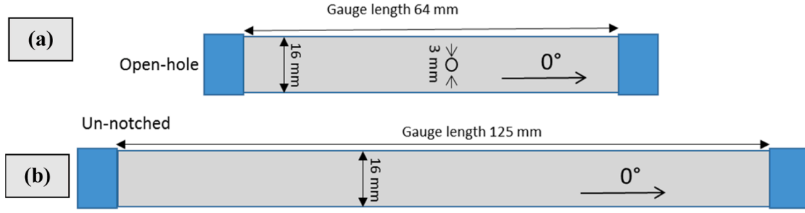
Fig. 3. Schematics of the a) Open-hole, and b) Un-notched specimens.
