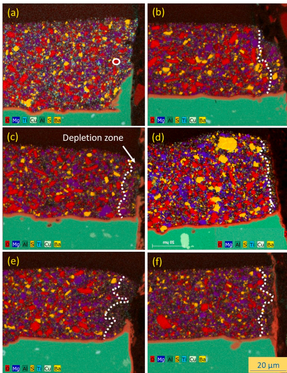
Fig. 6. EDS Quant maps of leaching. (a) 0 h, (b) 8 h, (c) 48 h, (d) 96 h, (e) 168 h and (f) 500 h exposure to NSS. The white circle in (a) encloses an example of a red particle which is shown later to contain Li (from PIGE) and is therefore assumed to be \text{Li}_2\text{CO}_3 indicating that all red particles are \text{Li}_2\text{CO}_3 . Colour coding for individual elements are included in the maps; the same code is used for all maps. Typical depletion zones are indicated by the dashed white lines in (b) to (f) (For interpretation of the references to colour in this figure legend, the reader is referred to the web version of this article).
