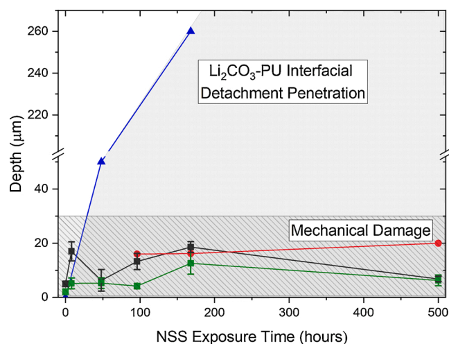
Fig. 7. Characteristic depletion/damage depths for different exposure times to NSS. ■ Depletion depth determined from SEM results, ● leaching penetration determined using first PIGE dataset, ■ leaching penetration determined using second PIGE dataset and ▲ deepest attack (PU-Li 2 CO 3 detachment observation) from SEM ion beam sections. As can be seen in Fig. 6, the depth to which depletion occurs varies considerably. Error estimates of the depletion depth above reflect this variation in depth. The 30 μm depth of the damage region is based on Fig. 2 where damage in the top part of the primer is in the vicinity of 20 μm, but towards the interface with the AA2024-T3 reaches towards 40 μm. Note: error bars only reflect the error in measurement for these sections, other sections with different initial distributions of particles and different levels of damage will have their own characteristic depletion depths.
