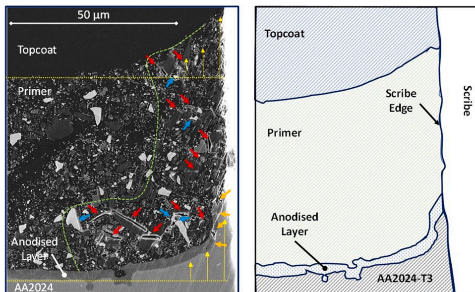
Fig. 2. Left - SEM image of deformation and damage at a section of scribe edge prior to any electrolyte exposure. Interfacial detachment has occurred at \text{Li}_2\text{CO}_3 particles (red arrows) and \text{BaSO}_4 particles (blue arrows). Orange arrows indicate cracking in the anodised layer. Yellow dashed lines indicate the baseline for the yellow arrows that show the level of deformation in the AA2024-T3. The green dashed line provides a rough indication of where damage has occurred. Right - Schematic of the image on the left including the position of the scribe edge and the scribe.
