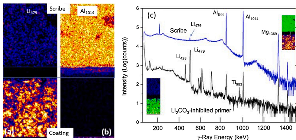
Fig. 4. PIGE results showing the presence of Li in the scribe after 500 h exposure to NSS. (a) Li map from the 479 KeV peak, (b) Al map from the 1014 keV peak and (c) respective spectra from the primer (under the topcoat) and the scribe. Bright green highlights where the spectrum was collected (either scribe or primer). The band between the two pale dashed lines in the centre of the maps indicates where there is an edge effect at the scribe. This is due to charge build-up in the coating (For interpretation of the references to colour in this figure legend, the reader is referred to the web version of this article.).
