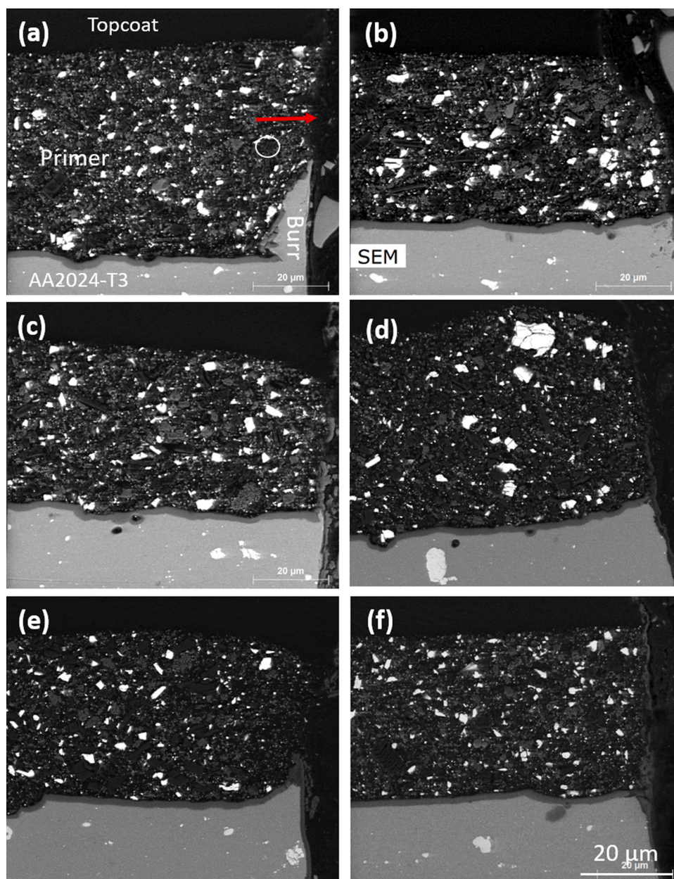
Fig. 5. SEM observations of leached primer as a function of time. (a) 0 h, (b) 8 h, (c) 48 h, (d) 96 h, (e) 168 h and (f) 500 h exposure to NSS. The red arrow in (a) indicates the direction of leaching. The white circle in (a) indicates a dark particle which is shown to be a \text{Li}_2\text{CO}_3 particle in analyses below (For interpretation of the references to colour in this figure legend, the reader is referred to the web version of this article).
