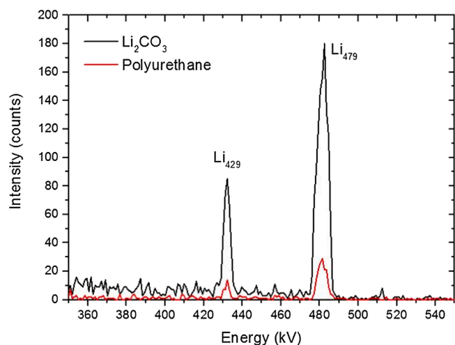
Fig. 10. PIGE spectra from \text{Li}_2\text{CO}_3 particle (black) highlighted by the white circles in Figs. 5, 6, 8 and 9 and adjacent polyurethane matrix (red) (For interpretation of the references to colour in this figure legend, the reader is referred to the web version of this article).
