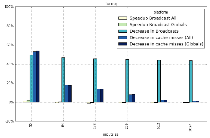
Fig. 7. Turing benchmark results
