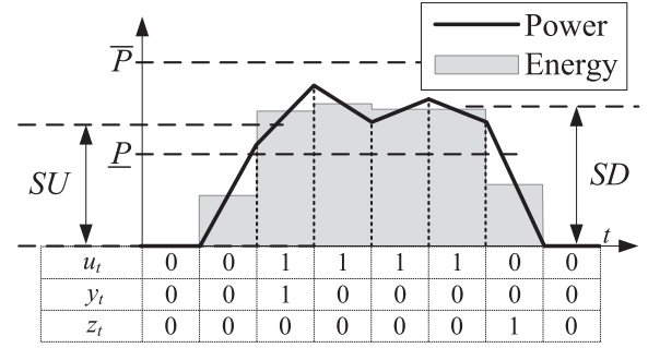
Fig. 6. Unit's operation under the power-based scheduling approach.
