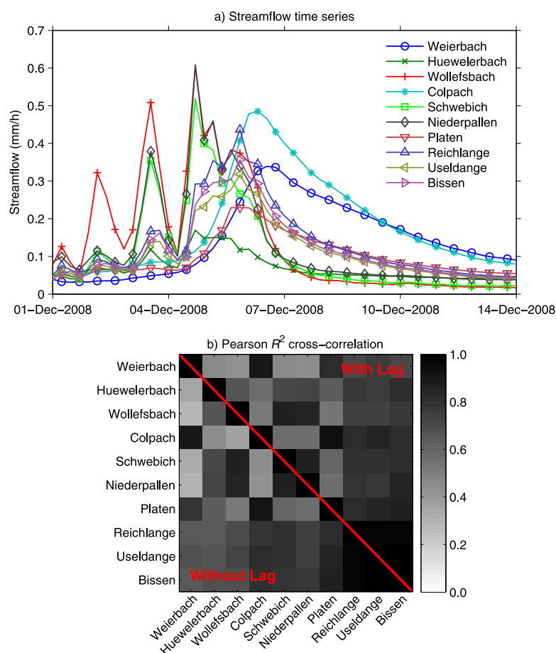
Figure 3. Streamflow diversity in the Attent catchment. (a) observed hydrographs over a 2 week period with a large storm event; (b) matrix of Pearson cross-correlation coefficients between the hydrographs of all subcatchments in the period 2000–2012. The lower triangle shows the R^2 between streamflows at the same time step (i.e., no lag), whereas the upper triangle shows the maximum R^2 computed over lags of 0 to \pm 4 days. The subcatchments are sorted from smallest to largest by area.
