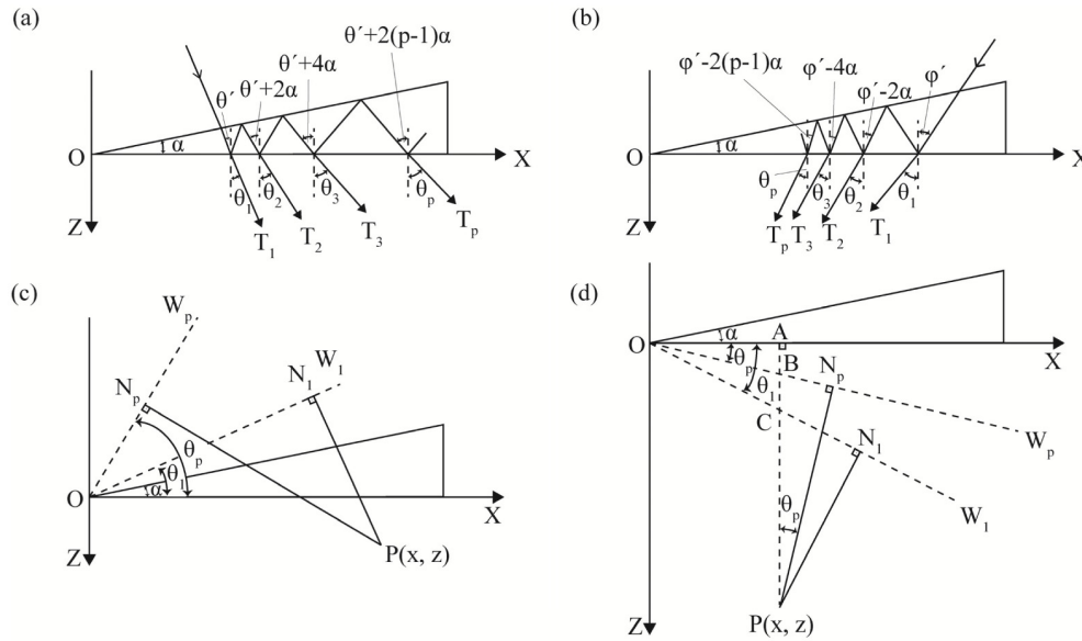
Fig. 4. Multiple reflections in a Fizeau interferometer at (a) positive and (b) negative incidence angle. Optical path difference after multiple reflections in a Fizeau interferometer at (c) positive and (d) negative incidence angle.
