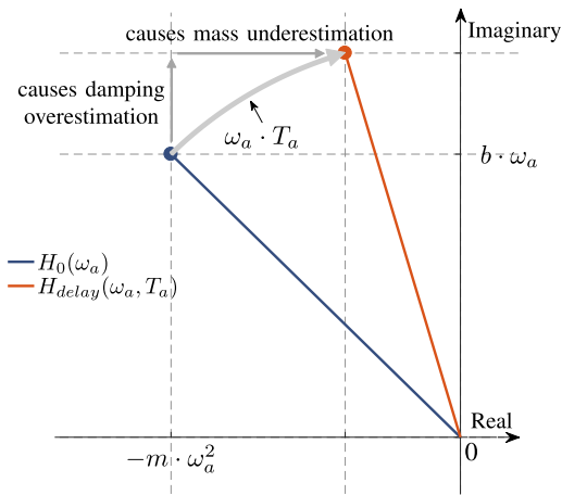
Fig. 6. Single-frequency Nyquist plots of a combined mass-damper system with undelayed force feedback (blue vector) and T_a -second delayed force feedback (red vector).
