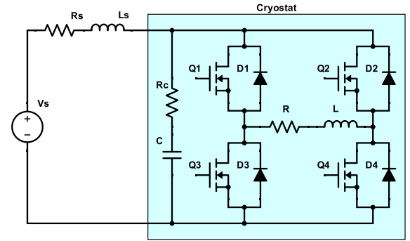
Fig. 1. Simplified schematic of the converter. During the short charge state, losses occur in the source equivalent resistance. During the much longer discharge state, there are almost no losses because of the low series resistance.
